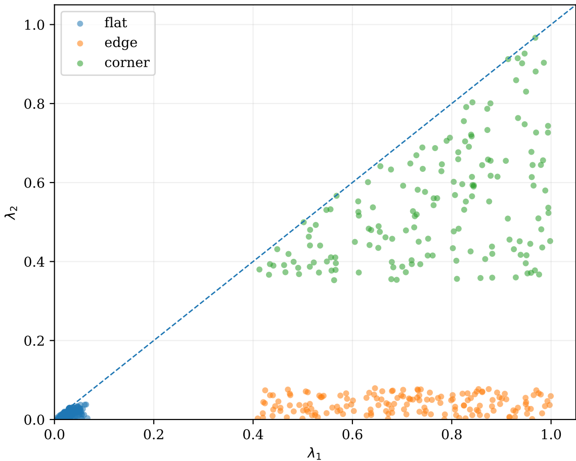
Local structure in the eigenvalue plane
