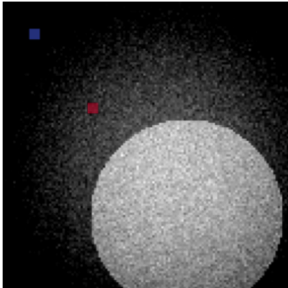
Seed labels
