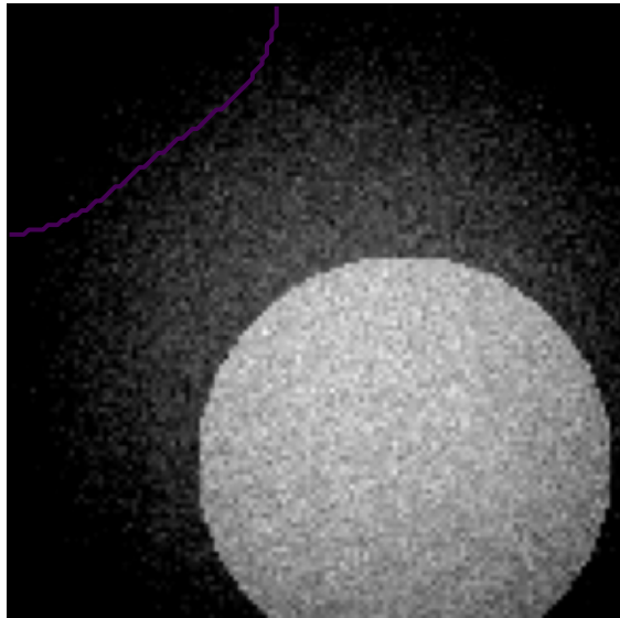
Harmonic boundary
