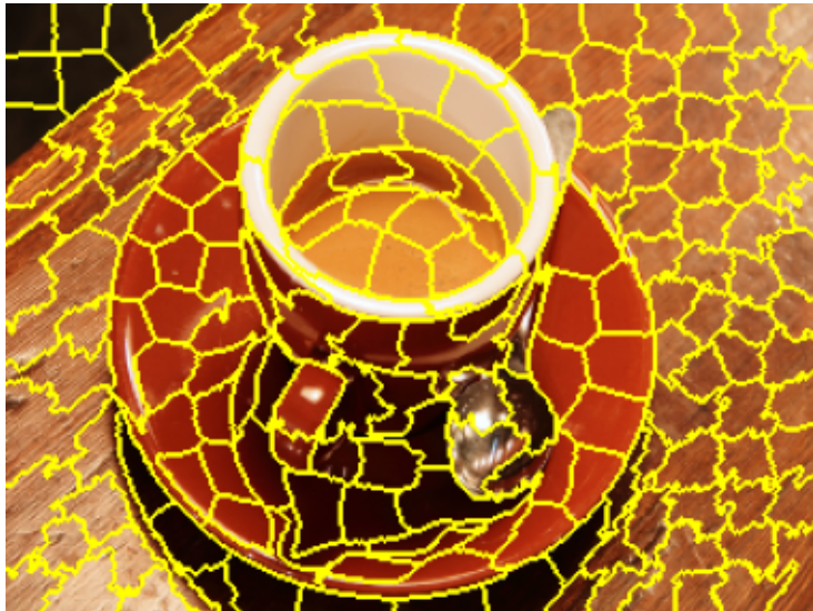
SLIC boundaries
