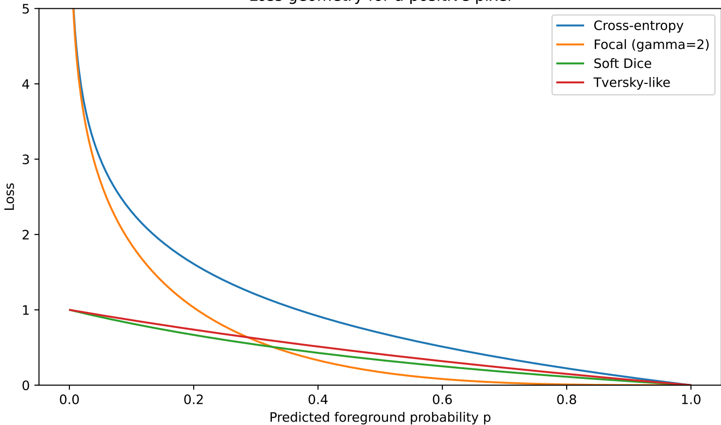
Loss geometry for a positive pixel
