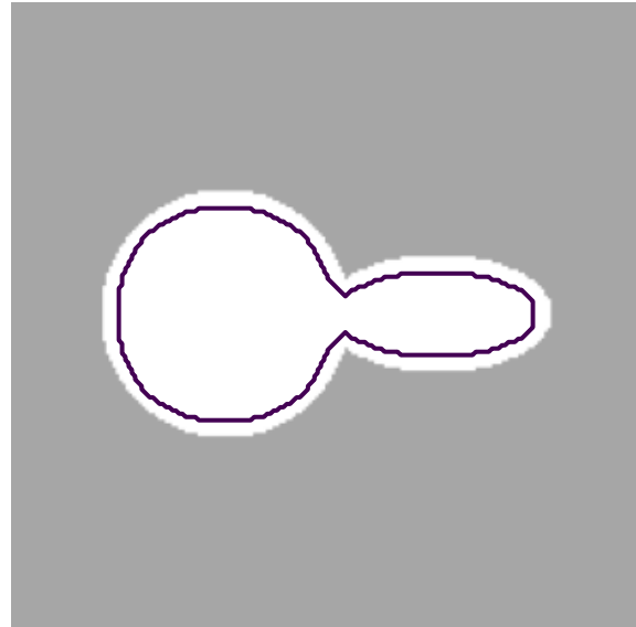
Boundary bias
