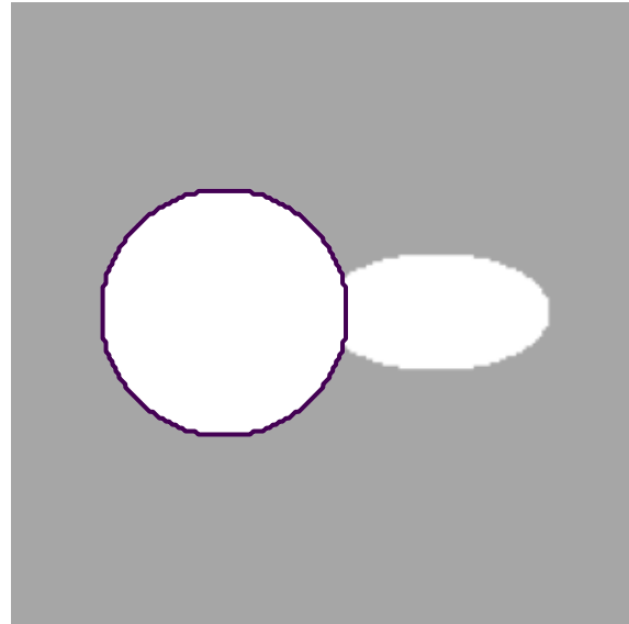
Small-object miss
