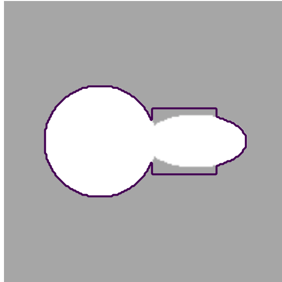
Leakage
