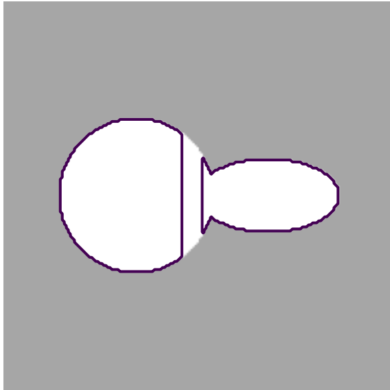
Fragmentation
