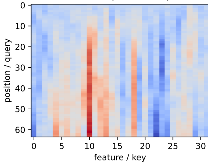
learned (illustrative)
