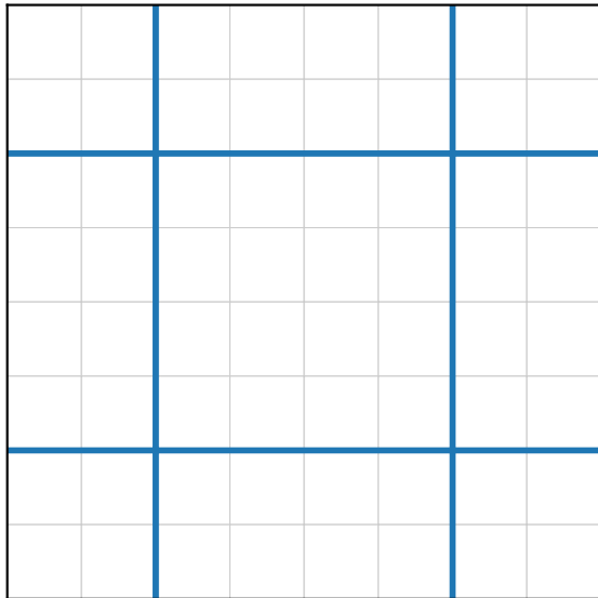
shifted-window attention
