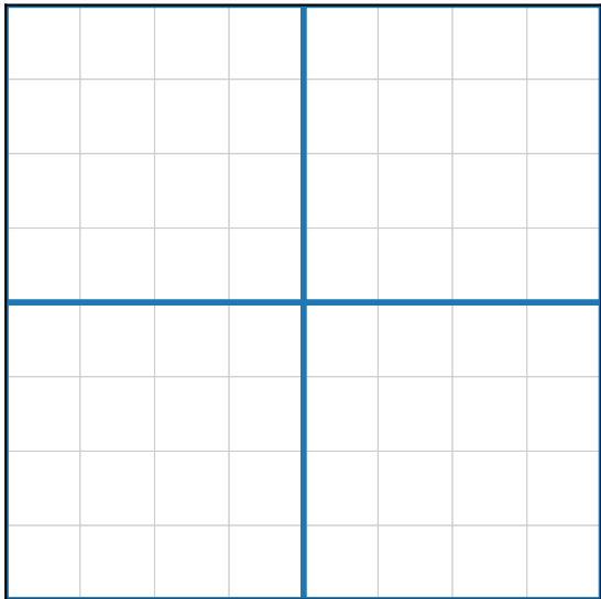
window attention
