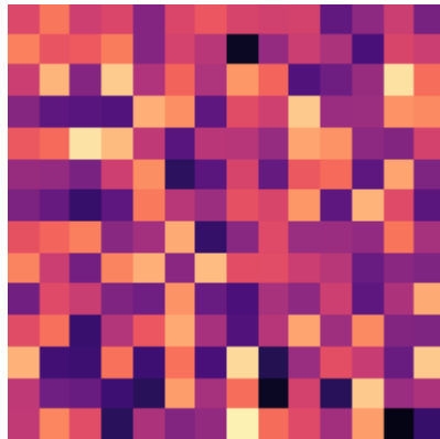
decoder reconstruction
