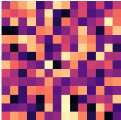
target patches
