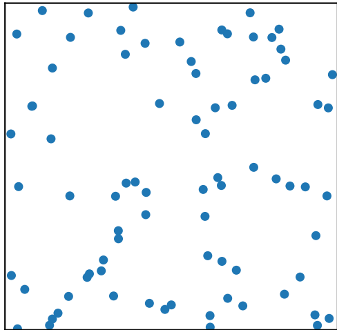
original tokens
