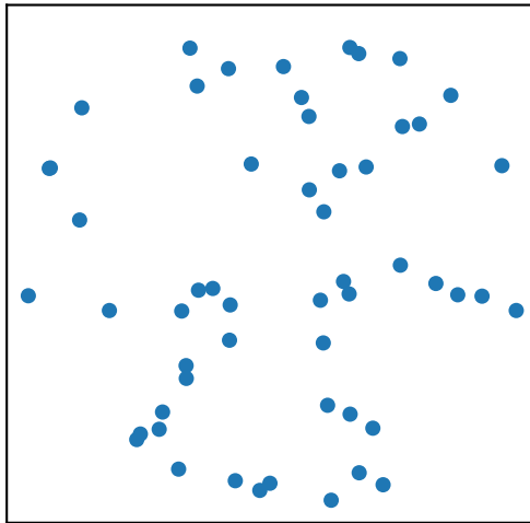
dynamic pruning
