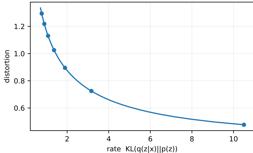
Rate-distortion frontier controlled by \beta
