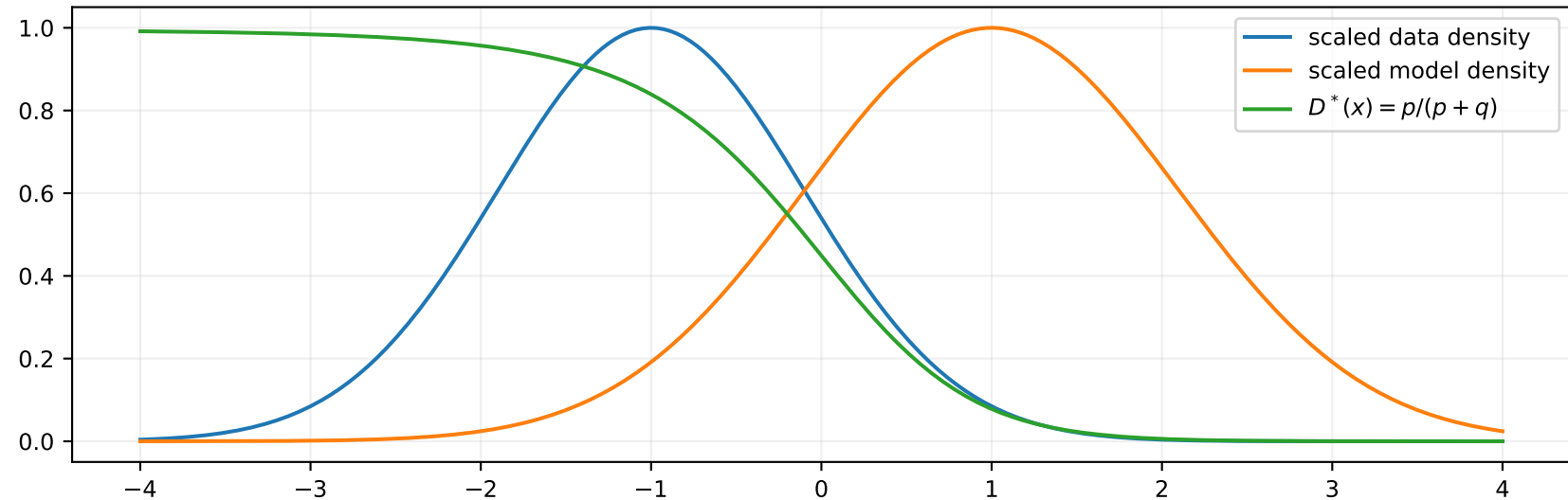
Optimal discriminator and density-ratio estimation
