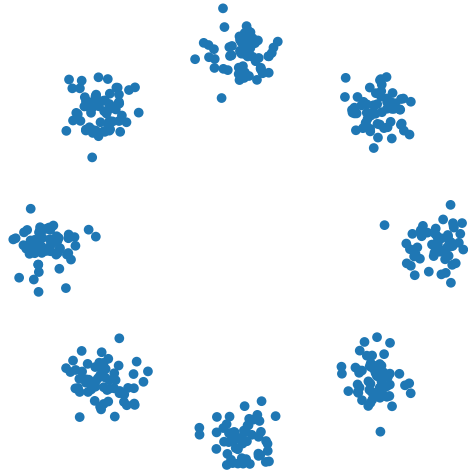
improved coverage
