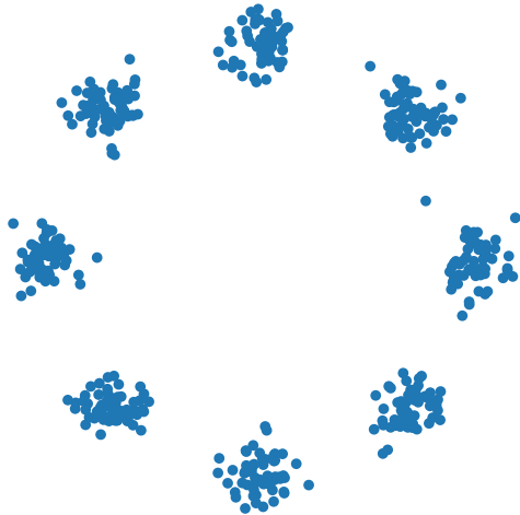
data modes
