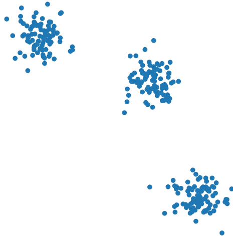
mode collapse
