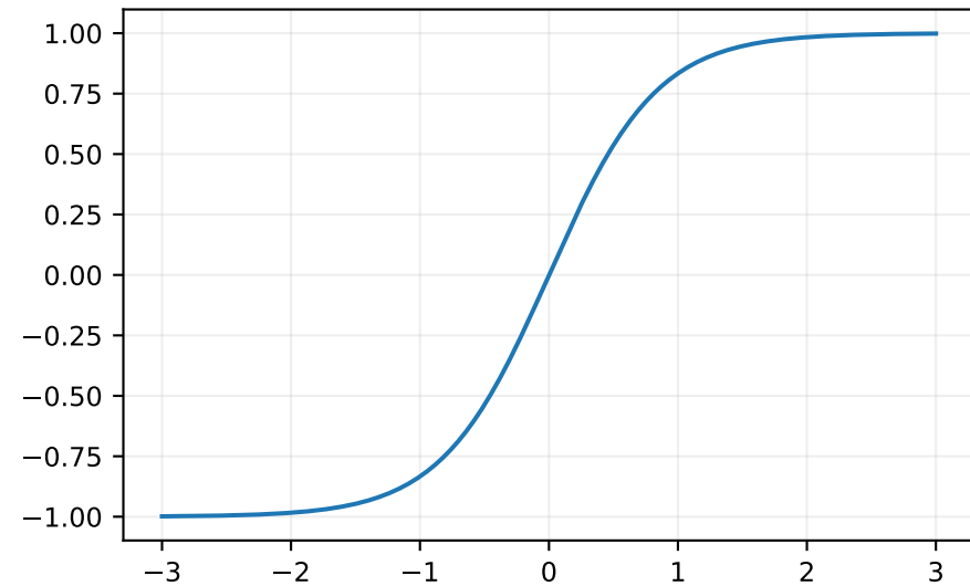
1-Lipschitz critic potential
