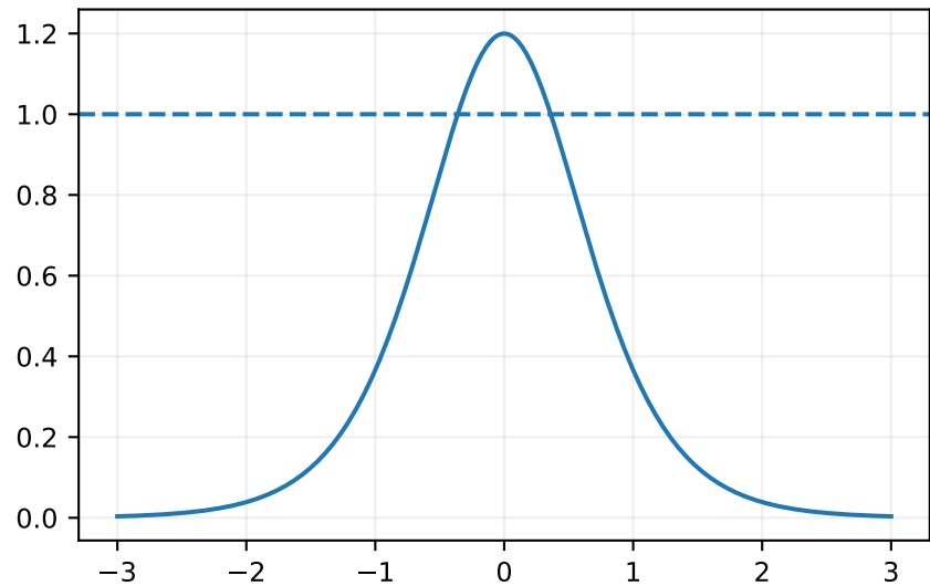
Gradient-norm regularization
