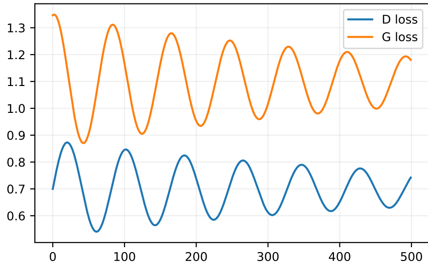
Losses can oscillate without indicating failure
