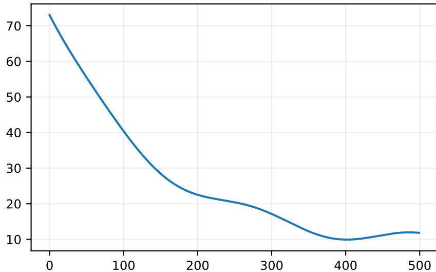
Use sample/coverage metrics and diagnostics
