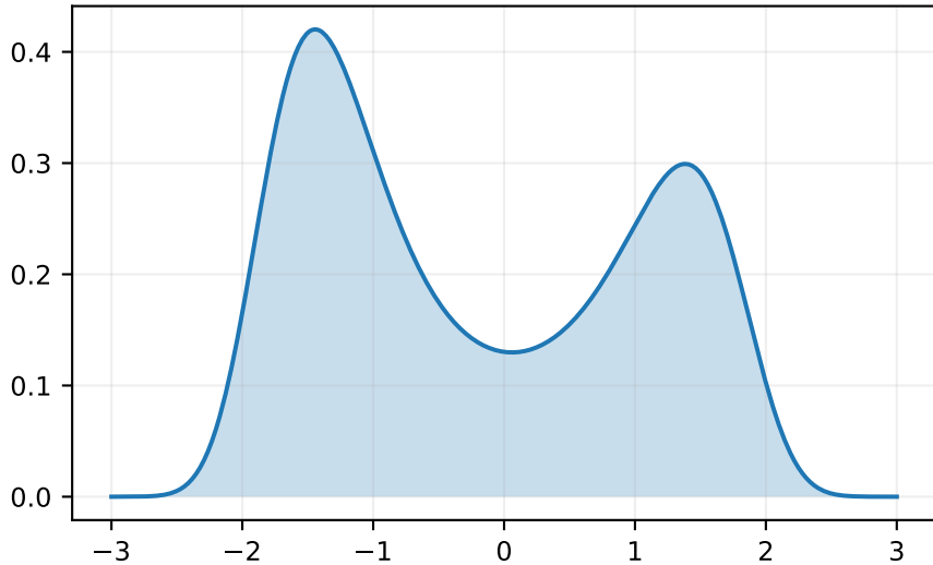
p_\theta(x) \propto e^{-E_\theta(x)}
