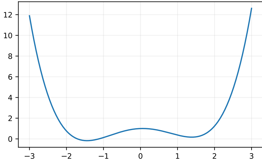
Energy E_\theta(x)
