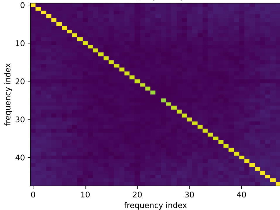
\log_{10} |FCF^*|
