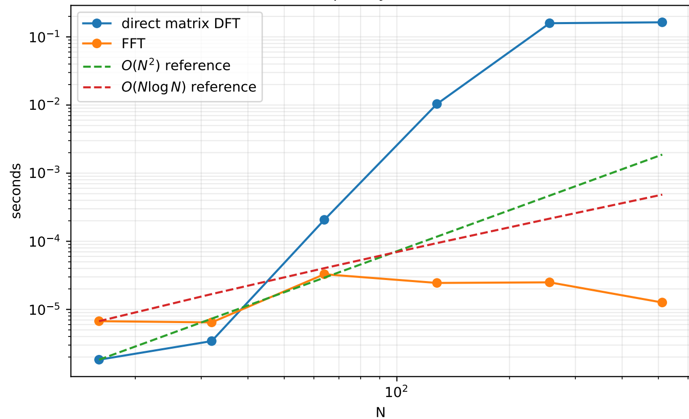
Measured complexity on the current CPU
