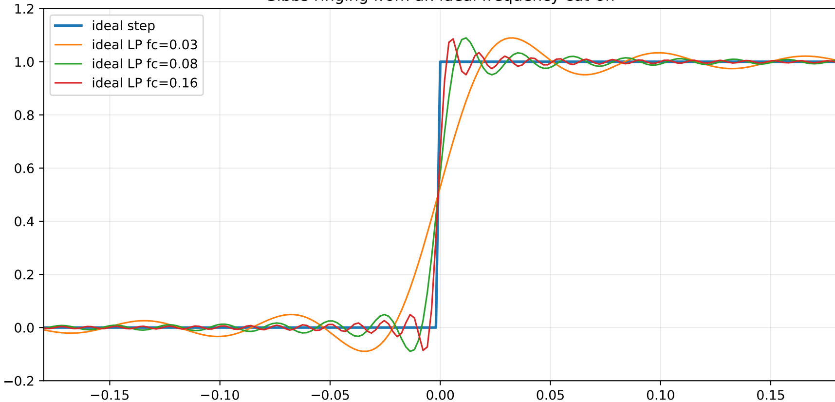
Gibbs ringing from an ideal frequency cut-off
