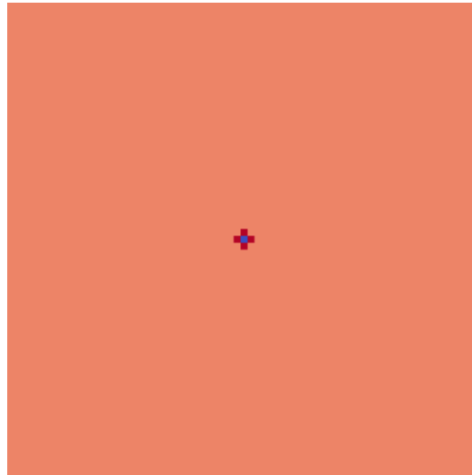
\log(1+|H|)
