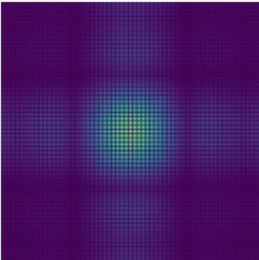
\log(1+|H|)
