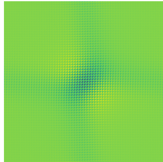
\log(1+|H|)
