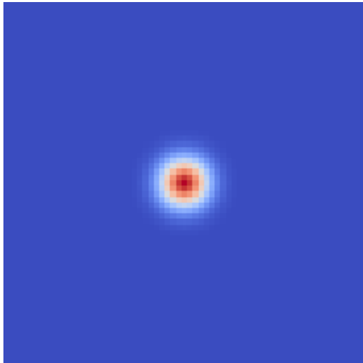
\log(1+|H|)
