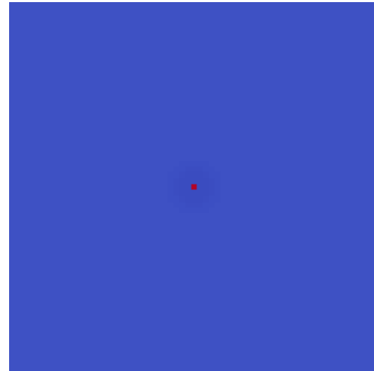
\log(1+|H|)
