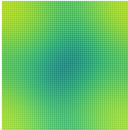
\log(1+|H|)
