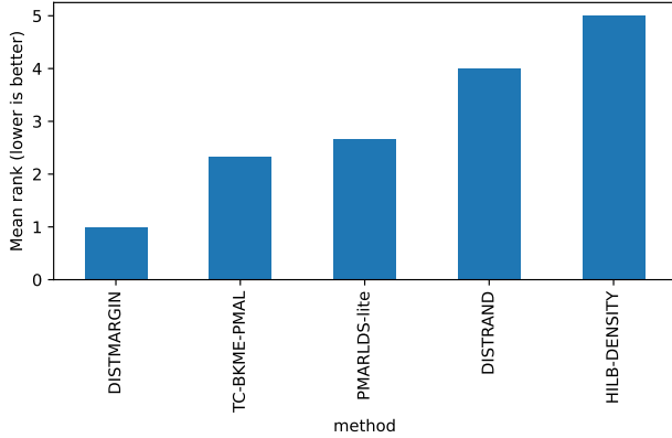
Fig. 2. Average-rank summary produced by the aggregation script for the smoke run. This diagnostic is included because the full paper should compare methods across several distributional tasks rather than relying on a single final-accuracy number.
