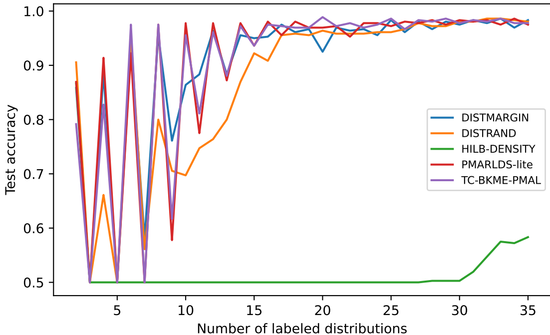
gaussdist variable
