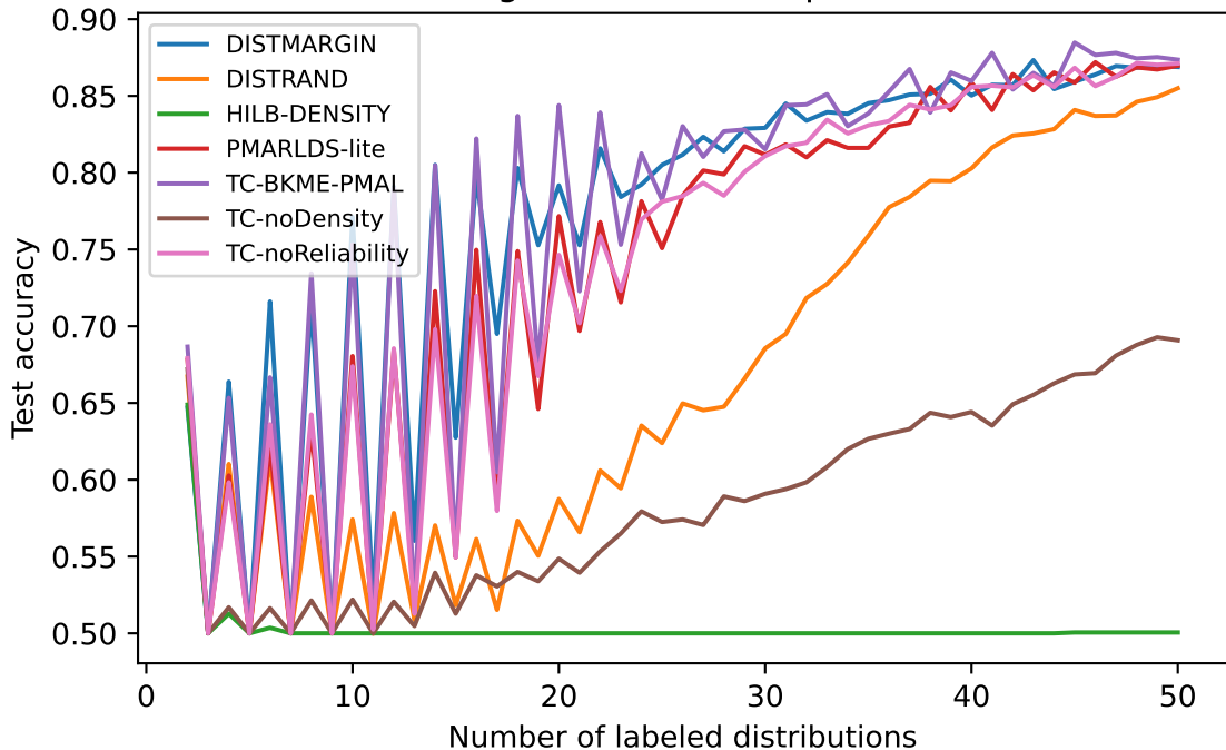
gaussdist hard equal
