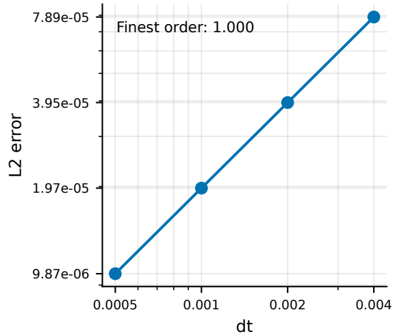
Explicit Euler
