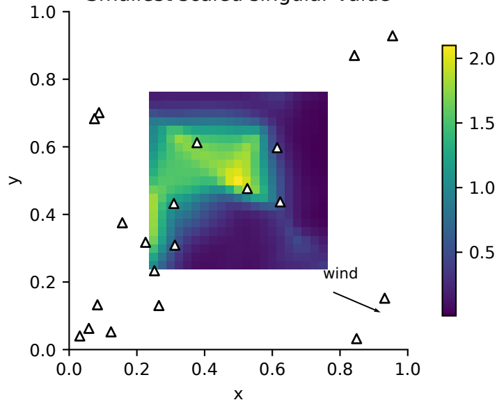
Smallest scaled singular value
