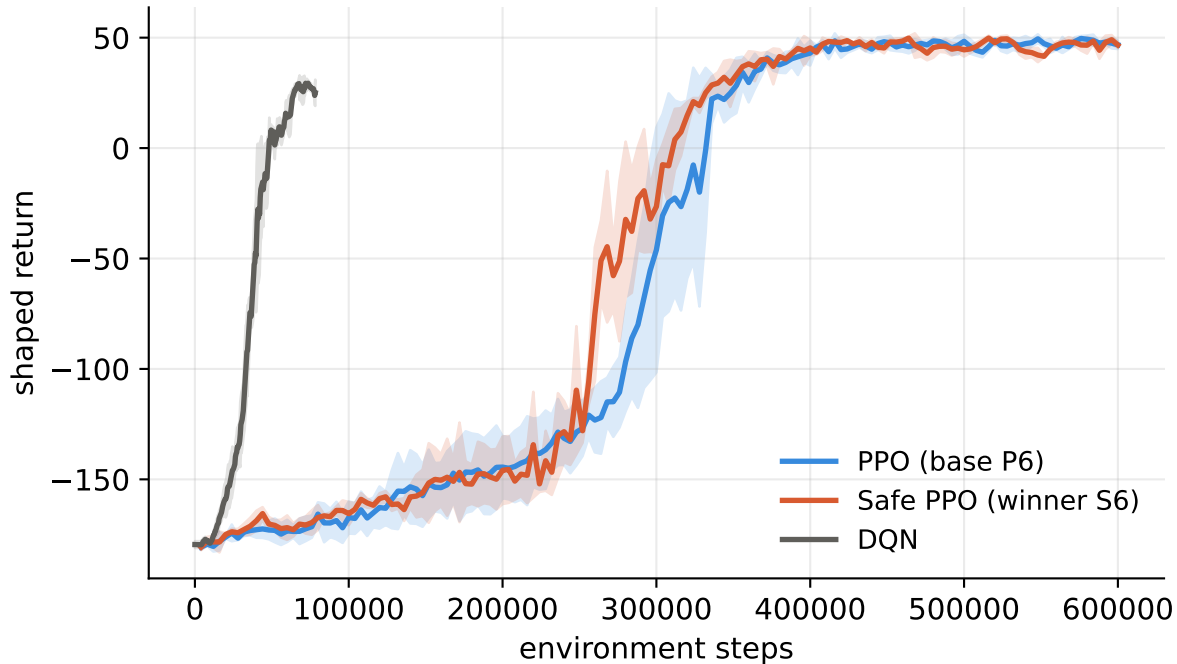
Learning curves (mean \pm std, 3 seeds)
