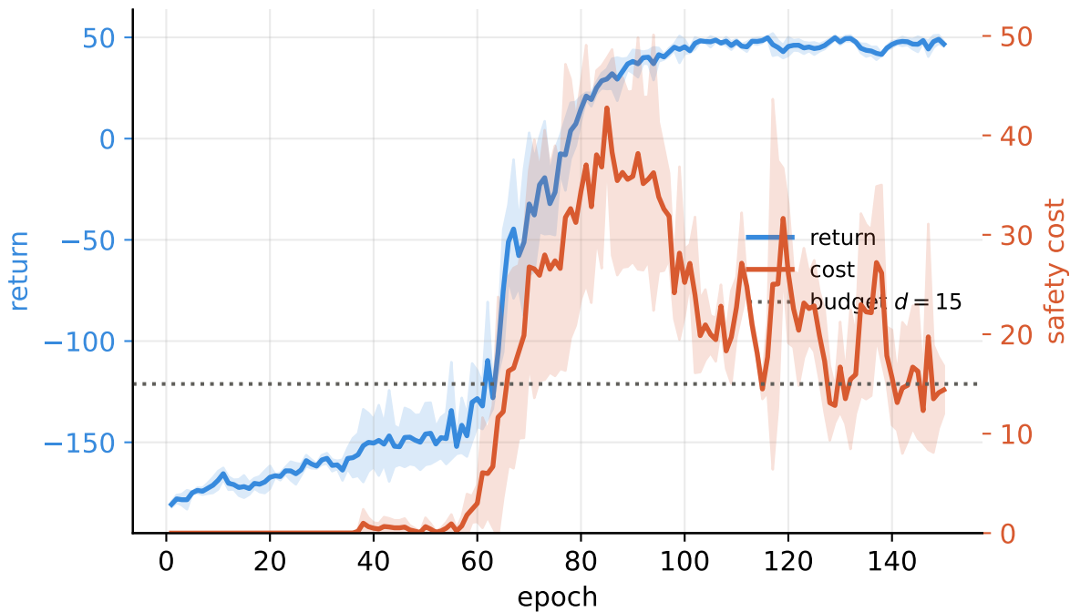
Safe PPO winner (S6): return and cost
