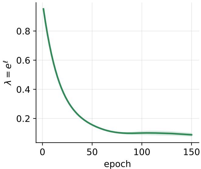
Lagrangian multiplier
