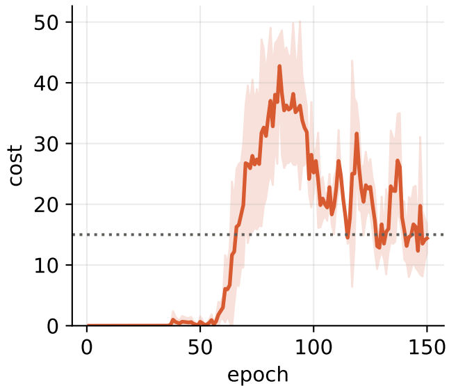
Safety cost vs. budget
