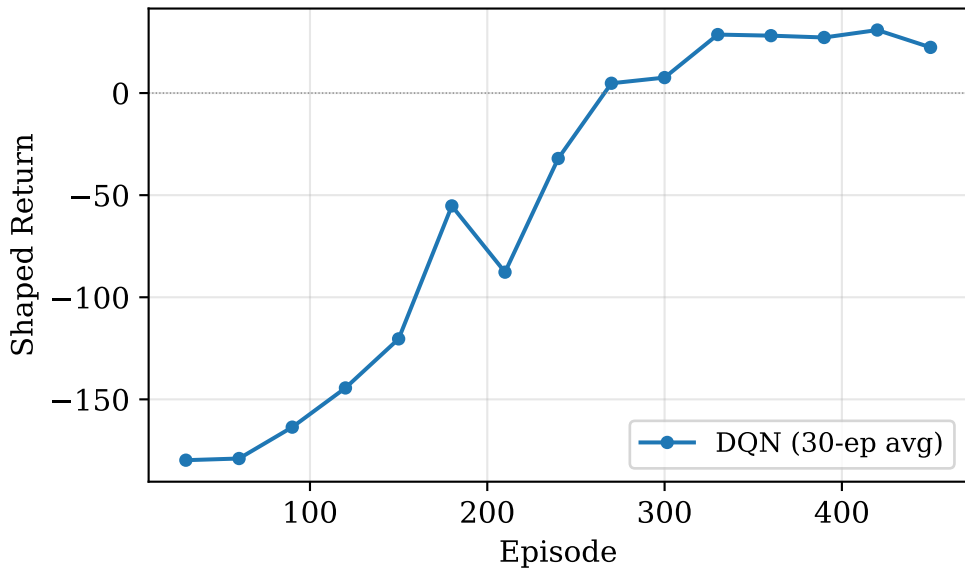
Phase 1: DQN Baseline Learning Curve
