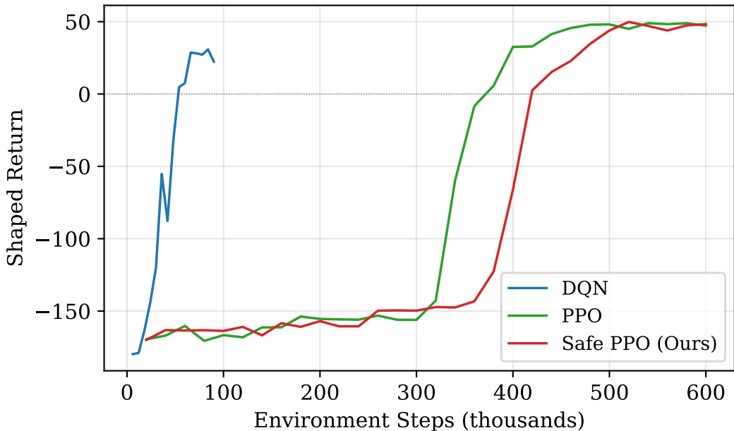
Return Comparison (1 seed)
