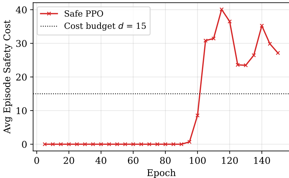
Safety Cost Trajectory under PPO-Lagrangian
