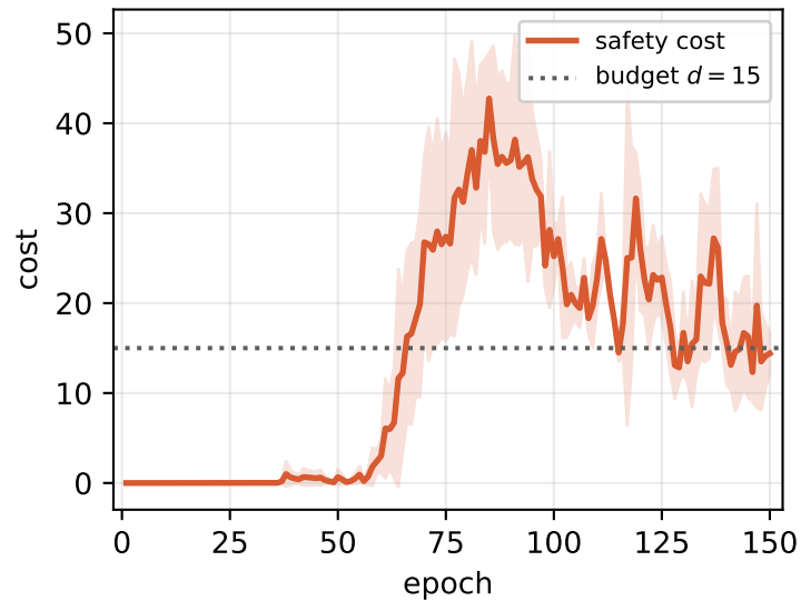
Safety cost
