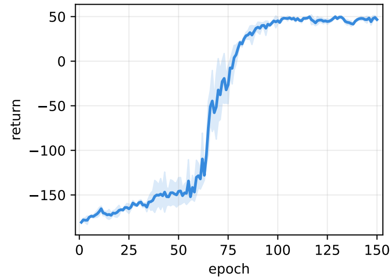
Shaped return
