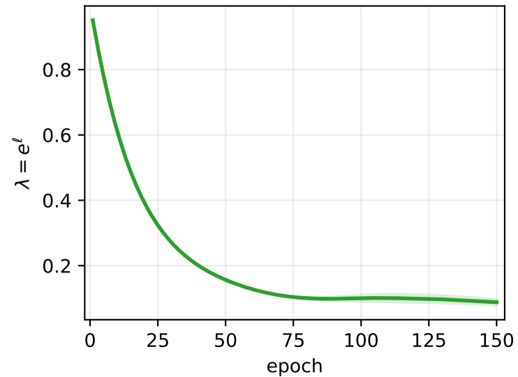
Lagrangian multiplier
