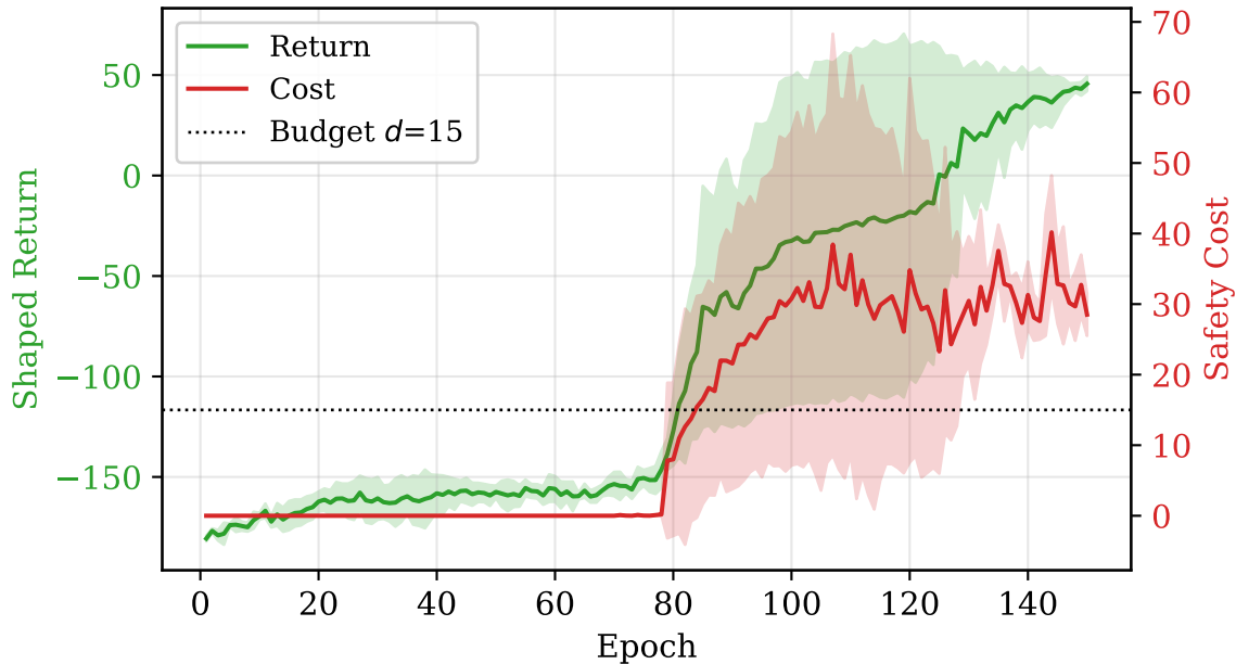
Safe PPO: Return vs Cost (3 seeds)
