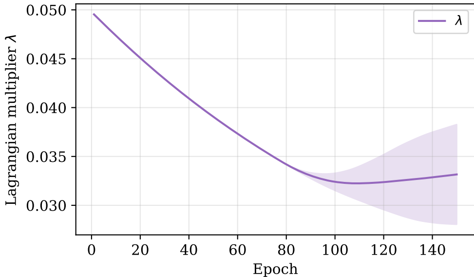
Adaptive \lambda Trajectory
