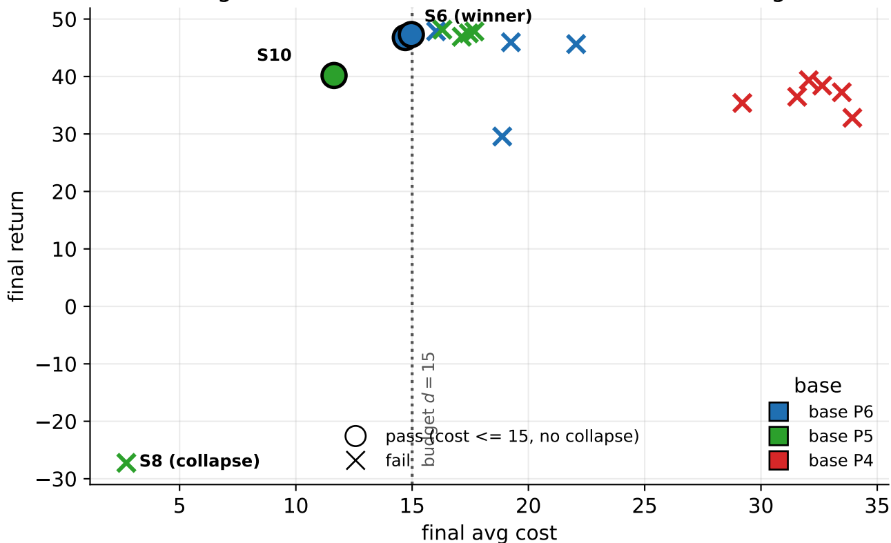
Stage 2: cost vs. return across 18 Safe-PPO configs
