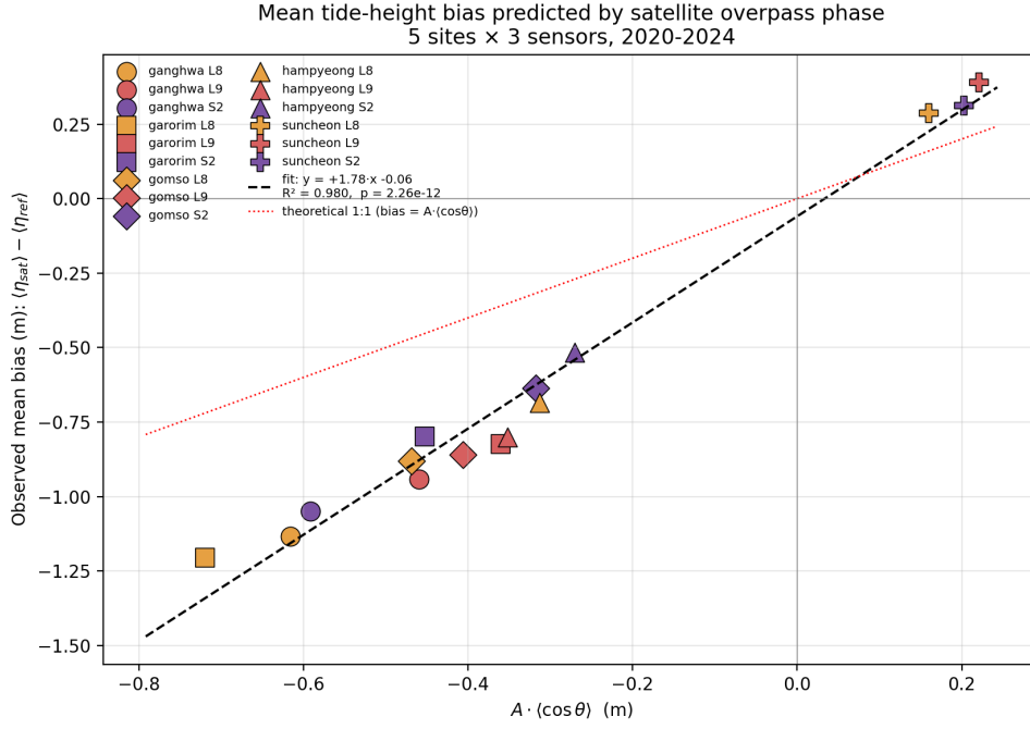
Figure 5. Measured mean tide-height bias versus the analytical predictor A \cdot \langle \cos \theta \rangle . Each of 15 points is one (site × sensor) pair. Marker shape encodes site, colour encodes sensor. Dashed black: OLS fit ( \beta = 1.78 , R^2 = 0.98 ). Dotted red: theoretical 1:1. A single parameter captures 98 % of the cross-site, cross-sensor variance, supporting the interpretation that the bias is set by satellite-overpass phase alone; the slope \beta > 1 is attributable to spring-neap covariance (Section 5.1).
