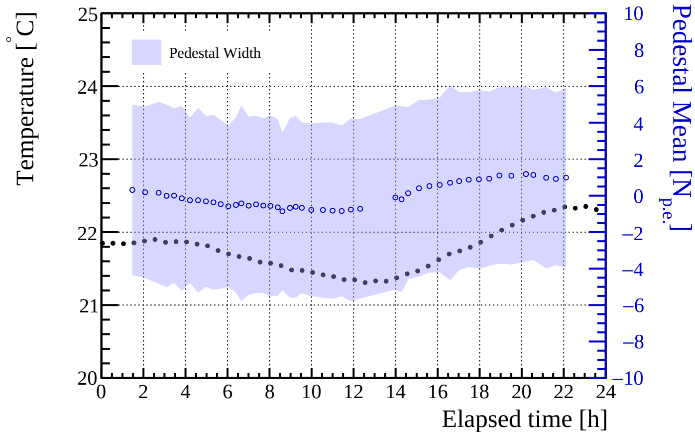
Temperature and BAC pedestal variation
