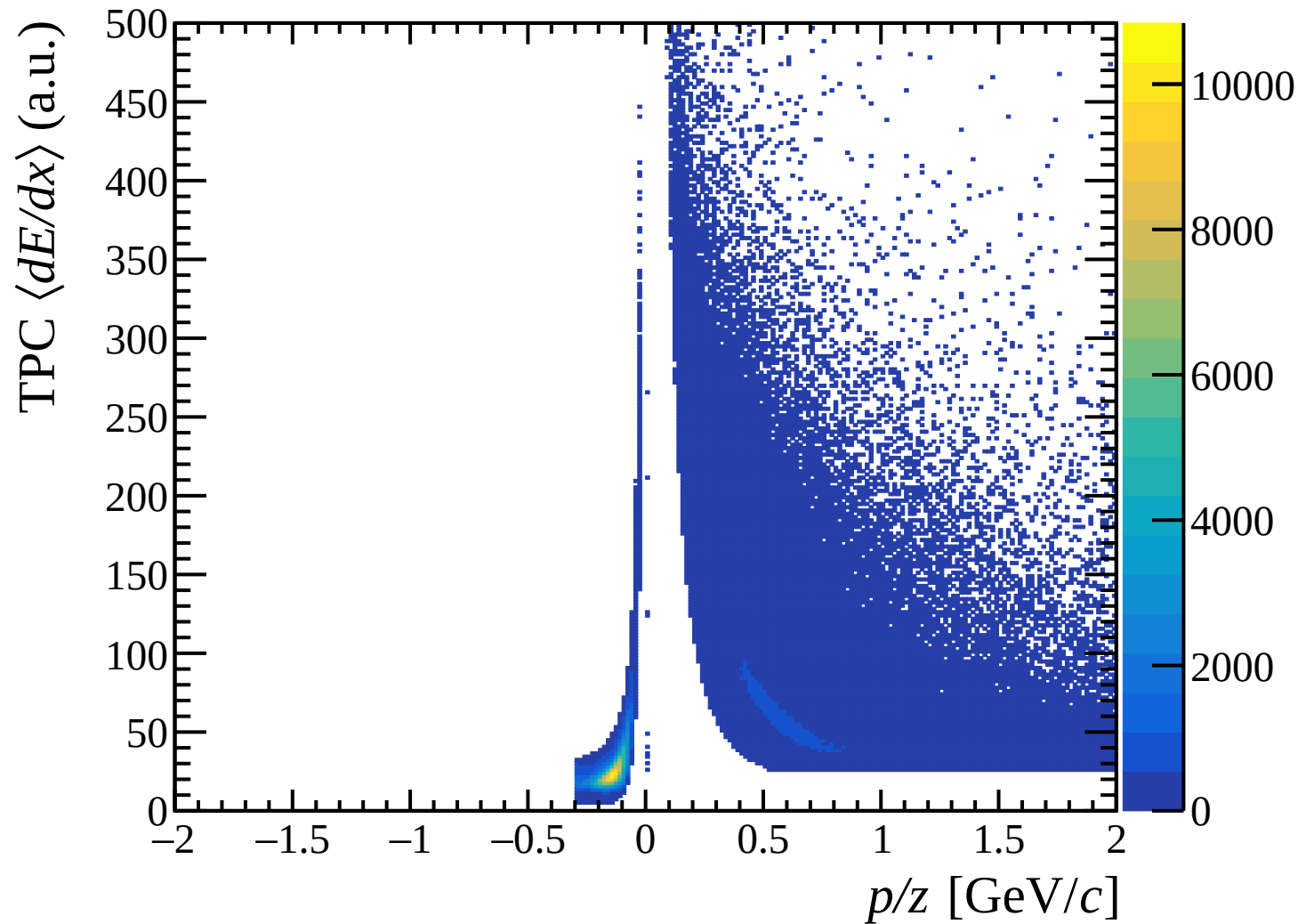
dE/dx vs signed momentum, tight cut
