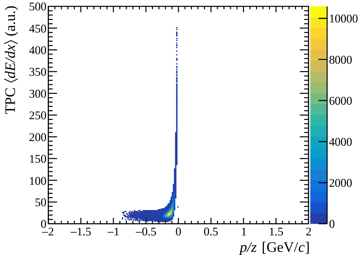
\pi^- dE/dx vs signed momentum, Lambda peak
