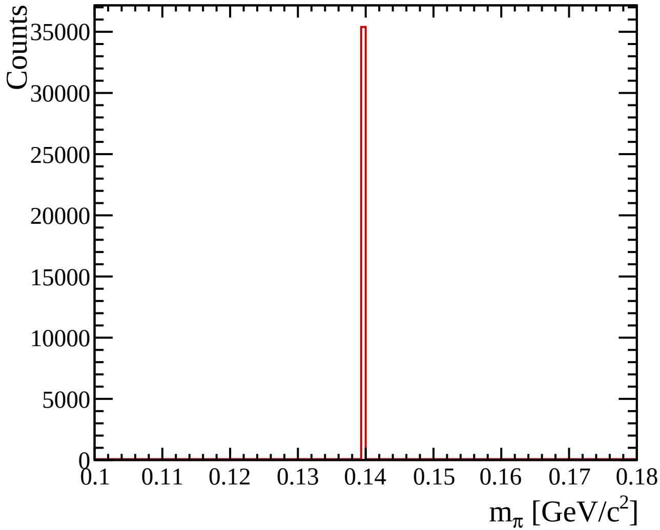
\pi^- candidate invariant mass, tight cut
