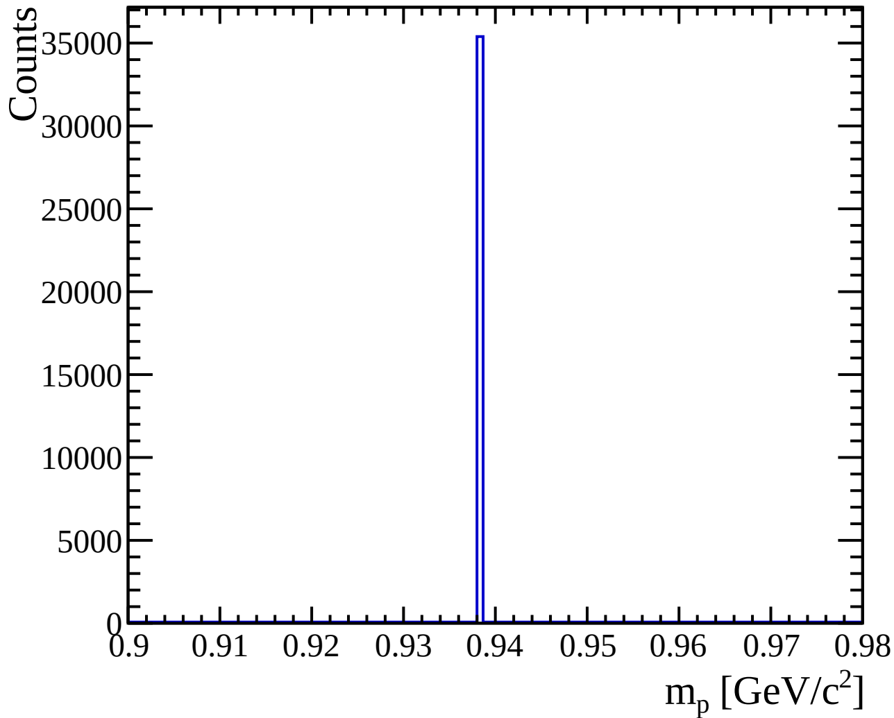
proton candidate invariant mass, tight cut
