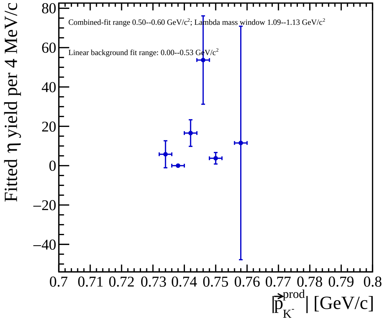
Gaussian-fit \Delta\eta yield vs production-vertex K^- momentum
