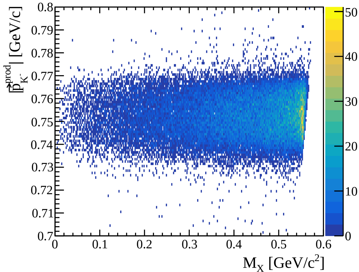
Production-vertex K^- momentum vs \Lambda\eta missing mass
