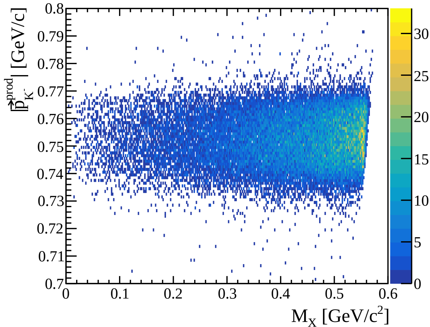
Production-vertex K^- momentum vs \Delta\eta missing mass
