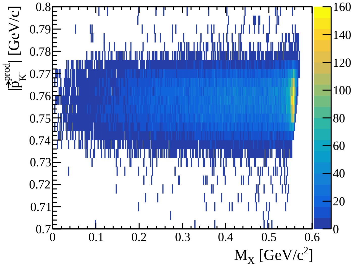
Missing mass vs production-vertex K18 momentum (no LH2 cut, no M_x cut)
