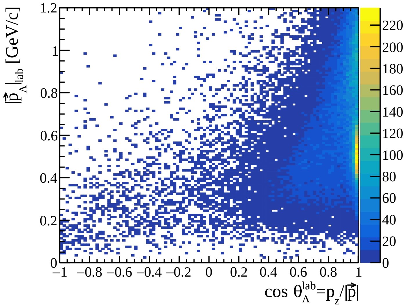
Selected \Lambda : lab \cos\theta vs lab momentum (no LH2 cut, all M_X )
