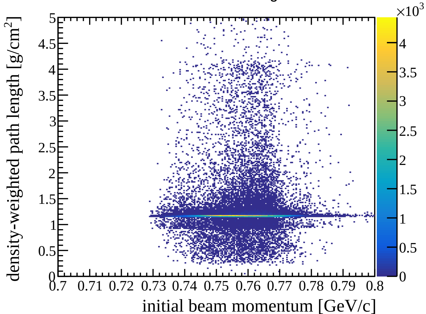
Initial beam momentum vs target thickness
