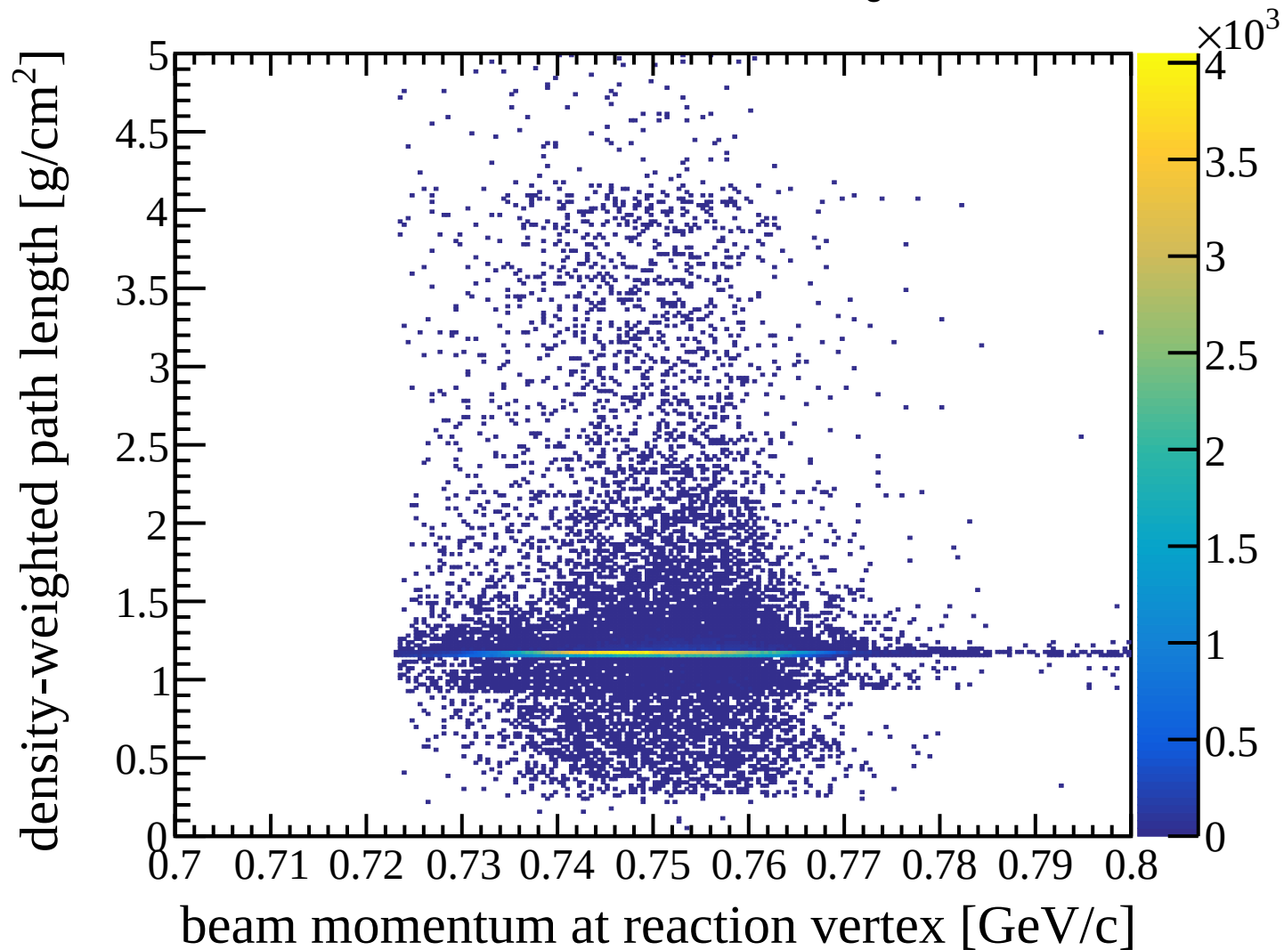
Reaction-vertex beam momentum vs target thickness
