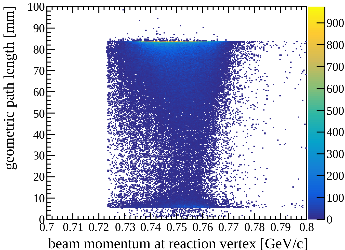
Reaction-vertex beam momentum vs geometric path length
