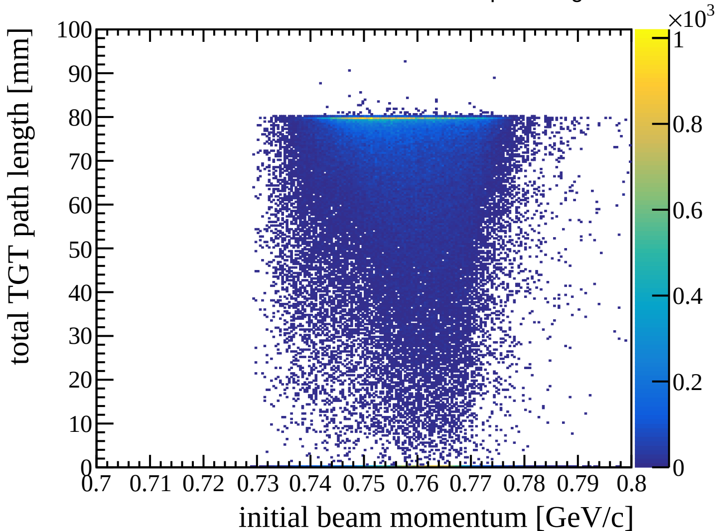
Initial beam momentum vs total TGT path length
