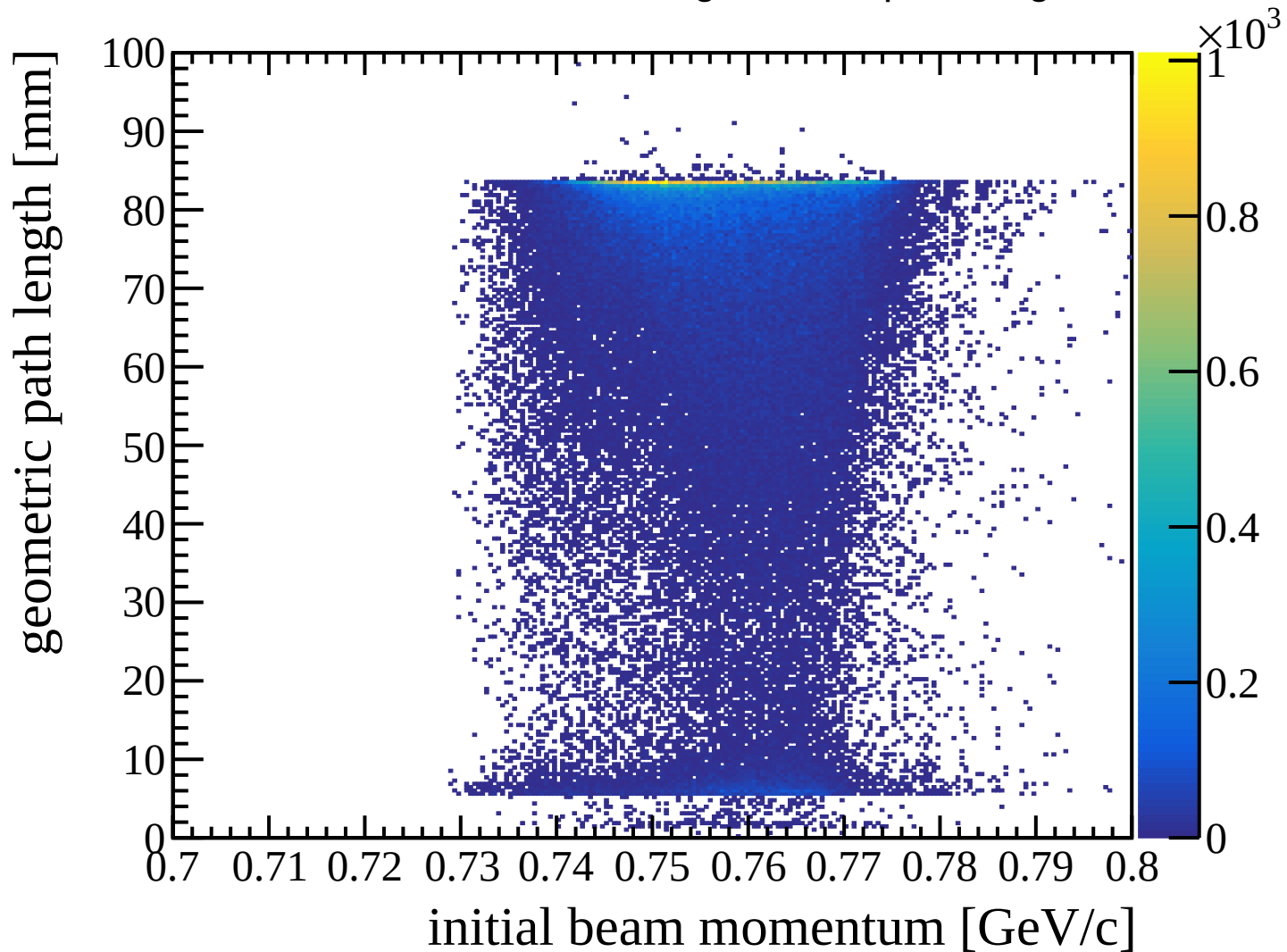
Initial beam momentum vs geometric path length
