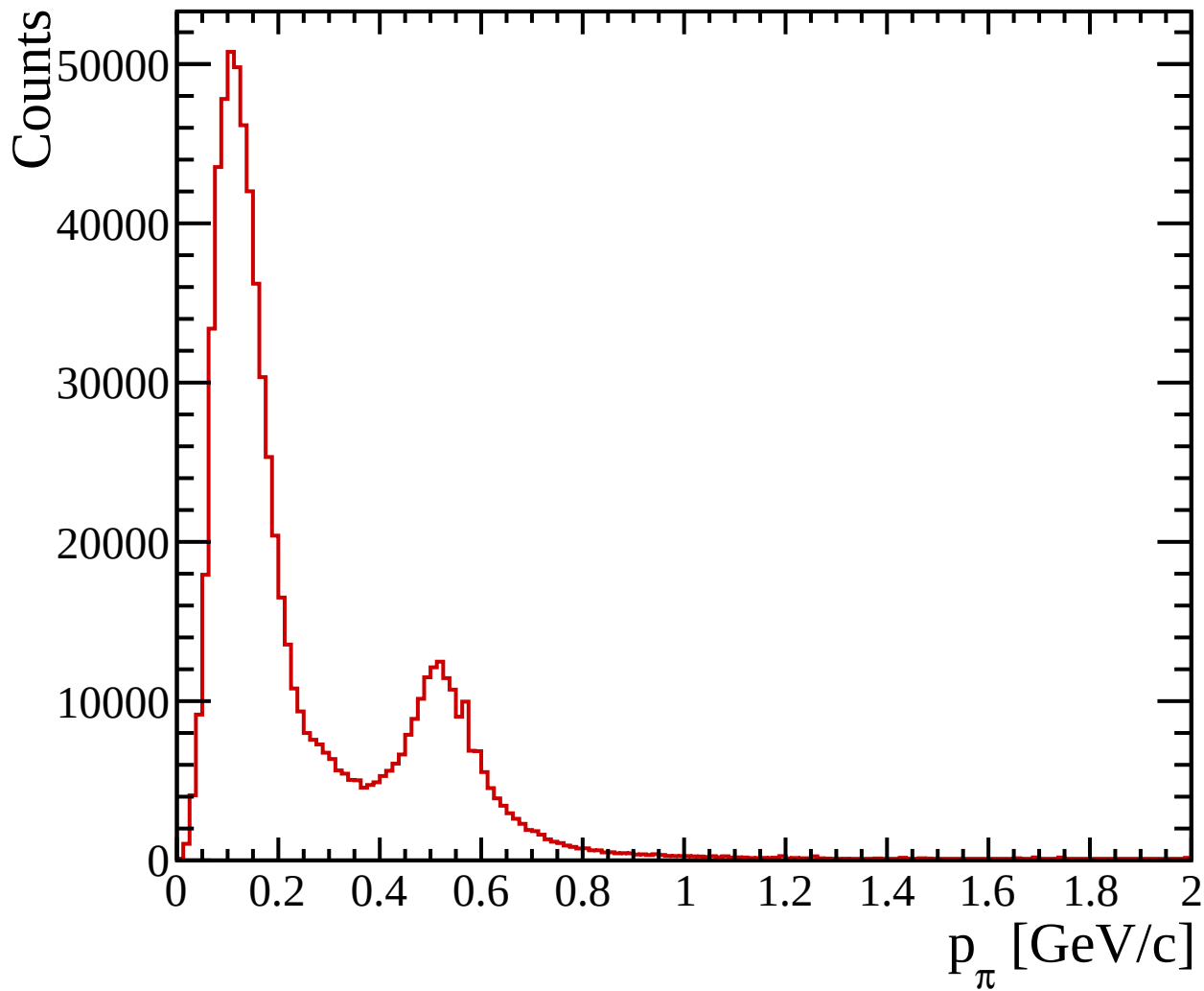
\pi^- momentum at mom0, tight cut
