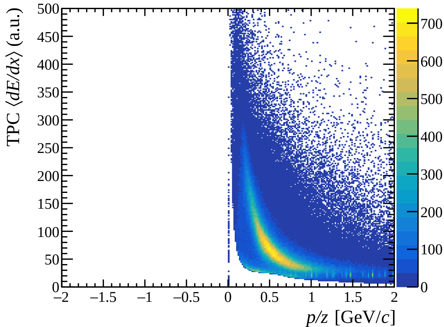
proton dE/dx vs signed momentum, tight cut
