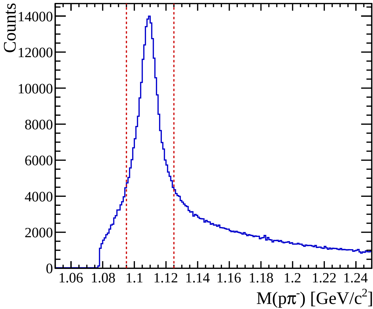
p\pi^- invariant mass, tight cut
