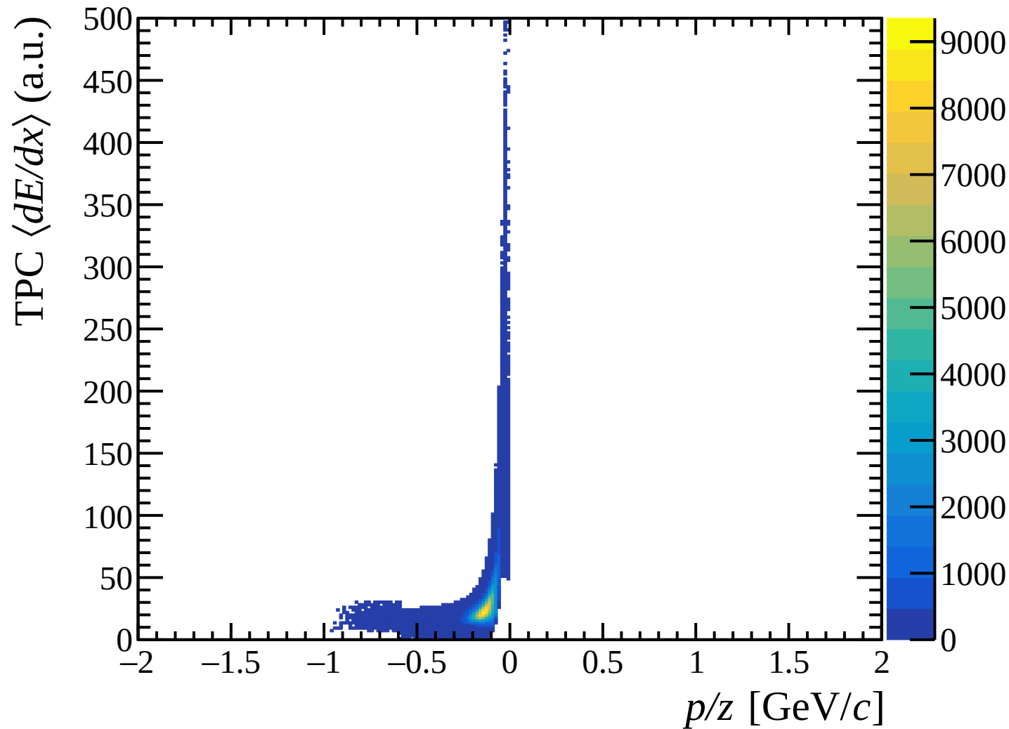
\pi^- dE/dx vs signed momentum, Lambda peak
