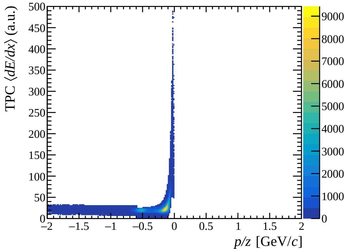
\pi^- dE/dx vs signed momentum, tight cut
