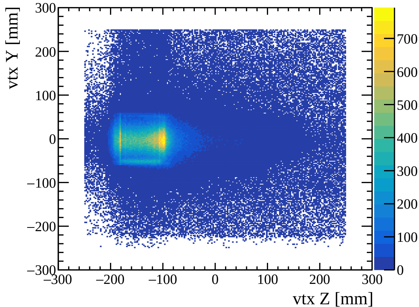
vertex, tight cut
