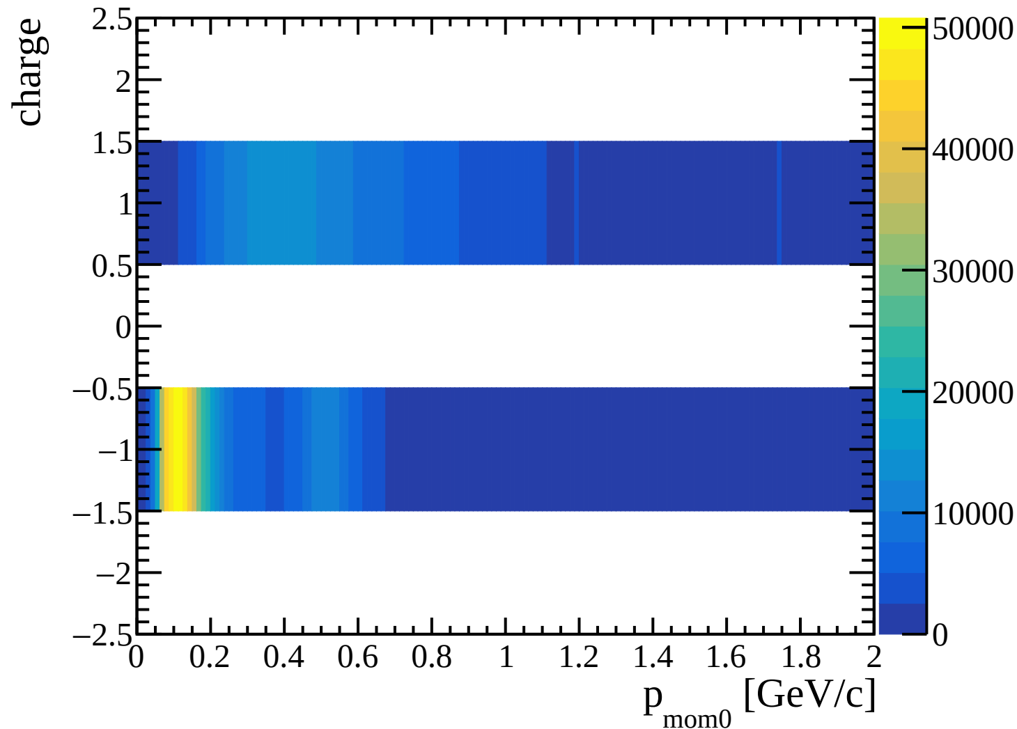
charge vs momentum, tight cut
