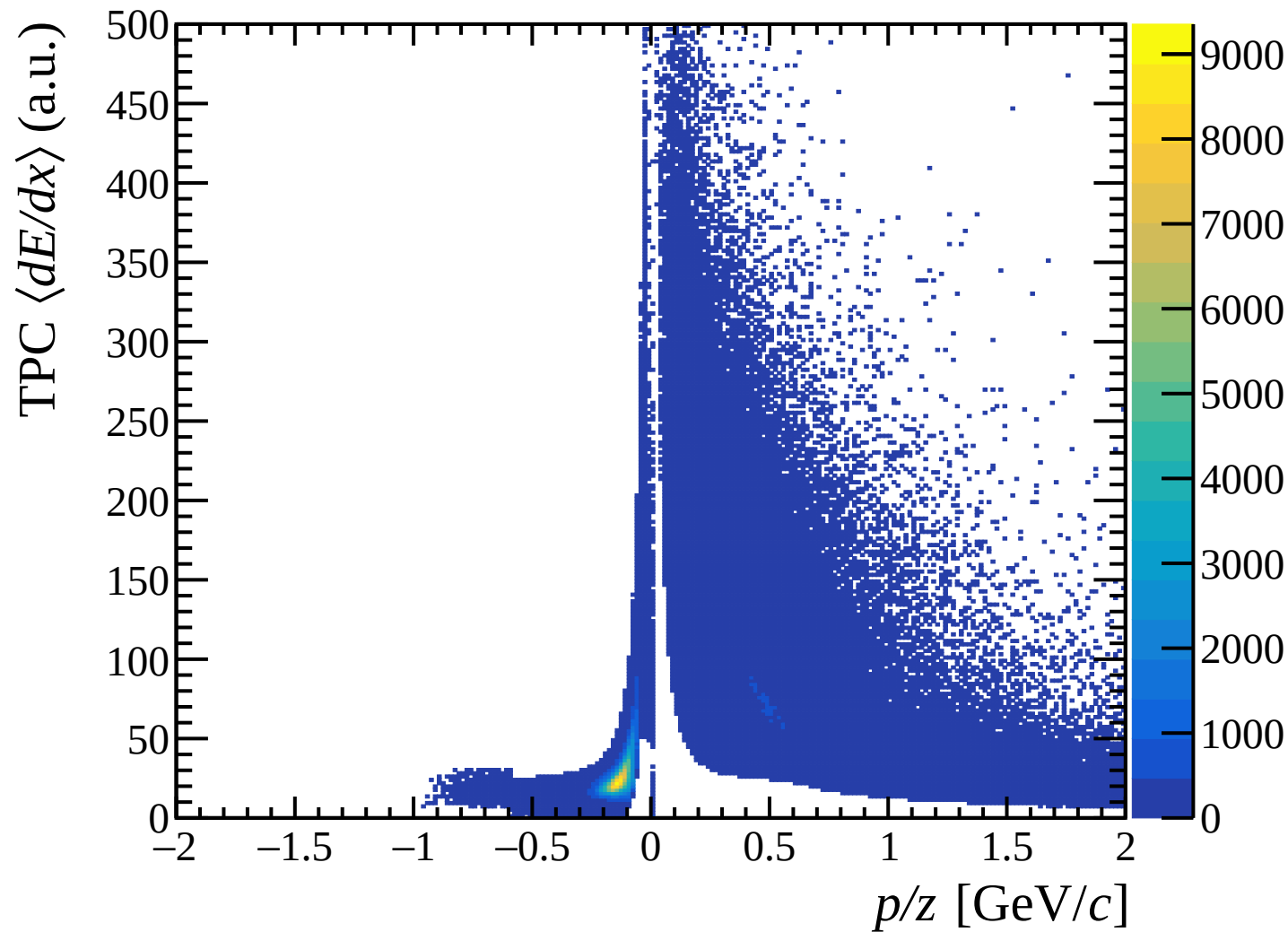
dE/dx vs signed momentum, Lambda peak
