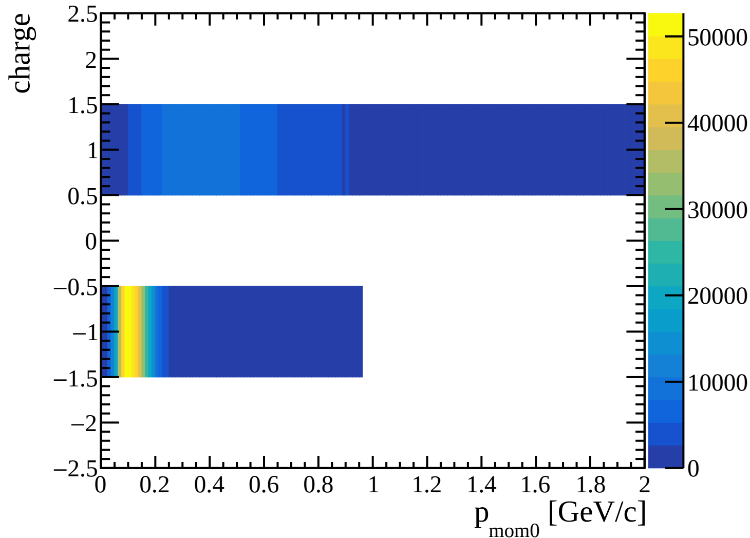
charge vs momentum, Lambda peak
