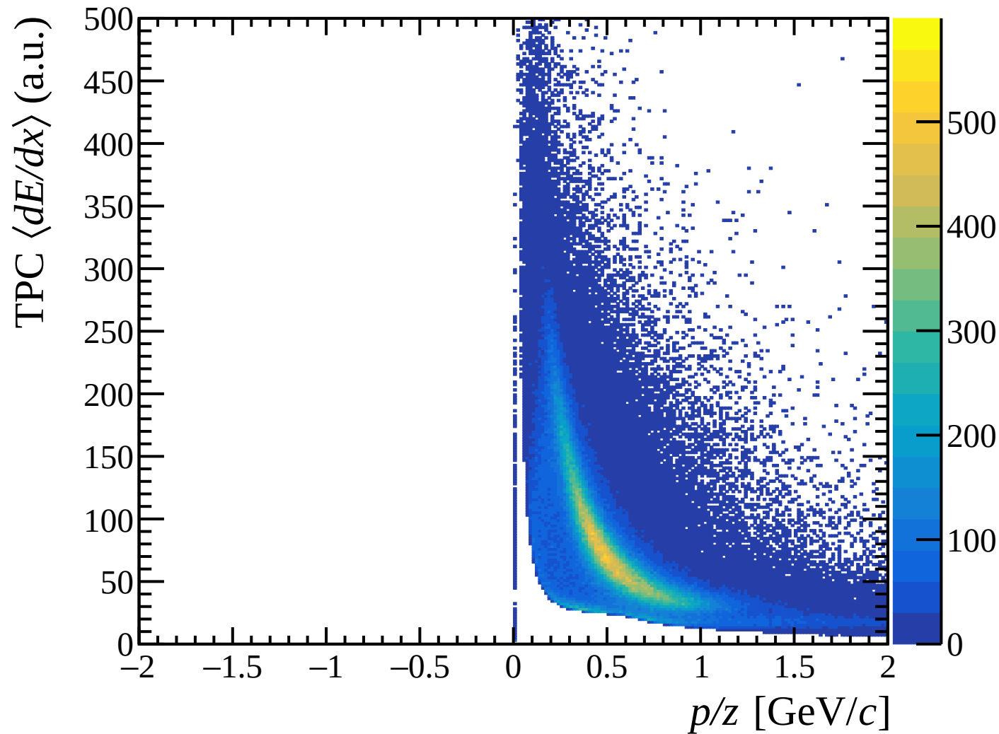
proton dE/dx vs signed momentum, Lambda peak
