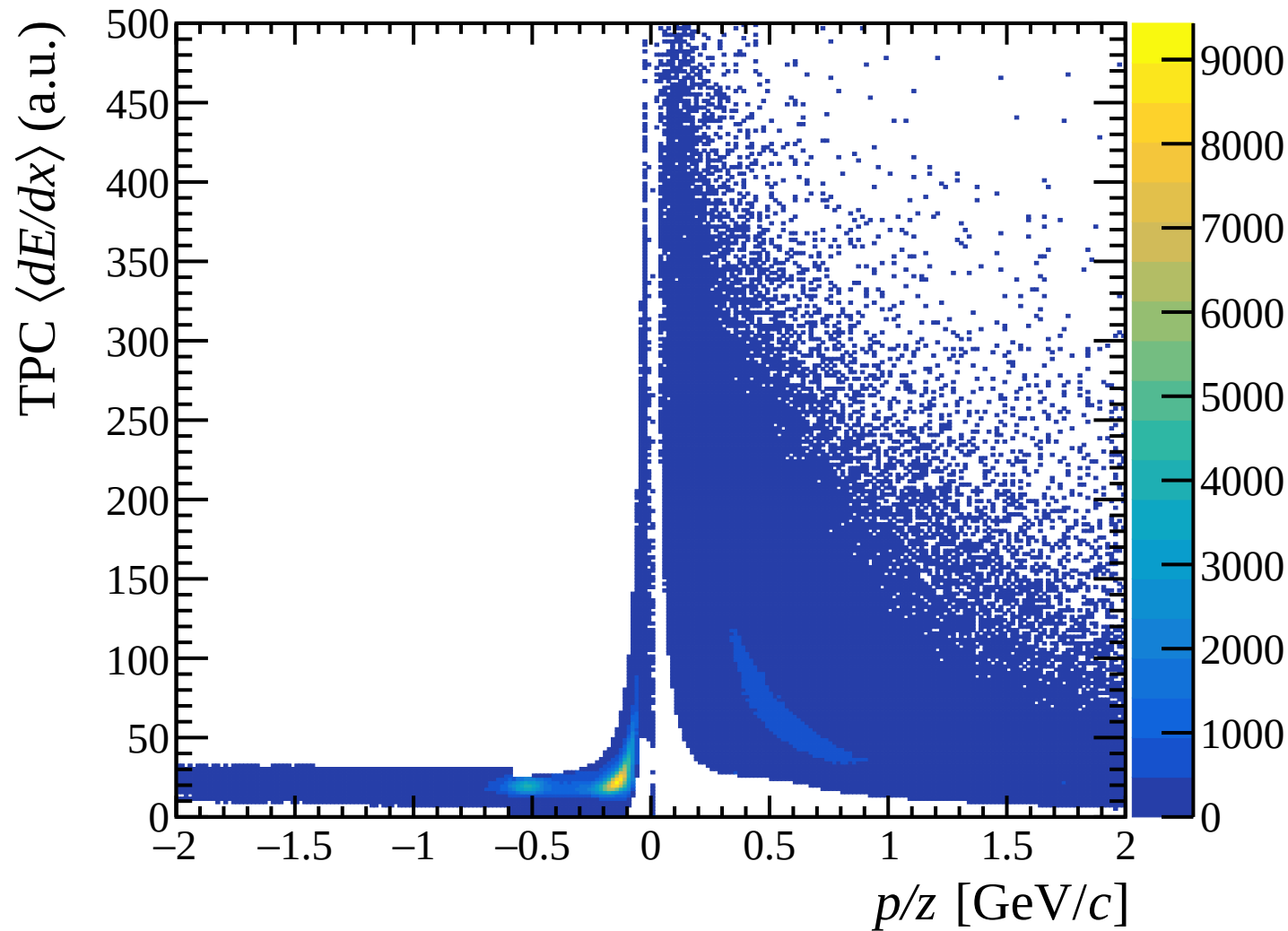
dE/dx vs signed momentum, tight cut
