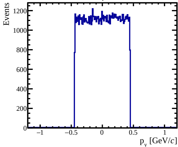
\pi^0 : p_y in lab
