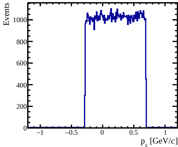
\pi^0 : p_z in lab
