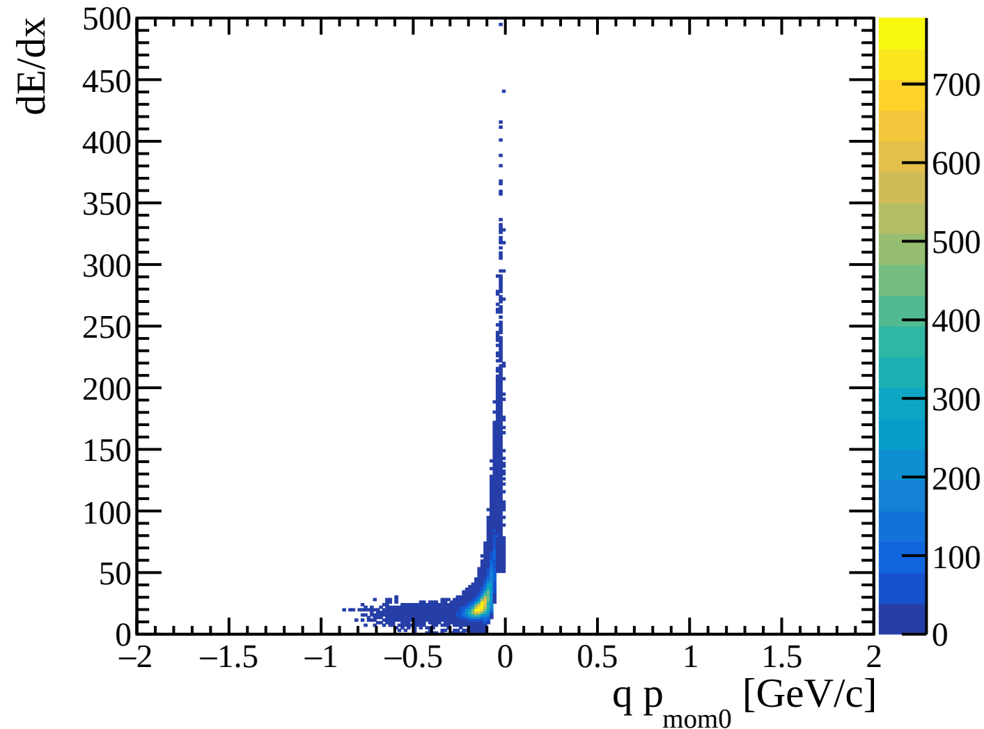
\pi^- dE/dx vs signed momentum, Lambda peak
