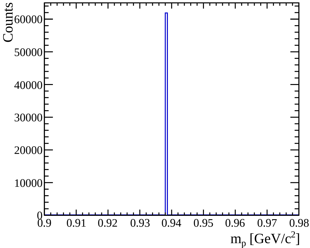
proton candidate invariant mass, tight cut
