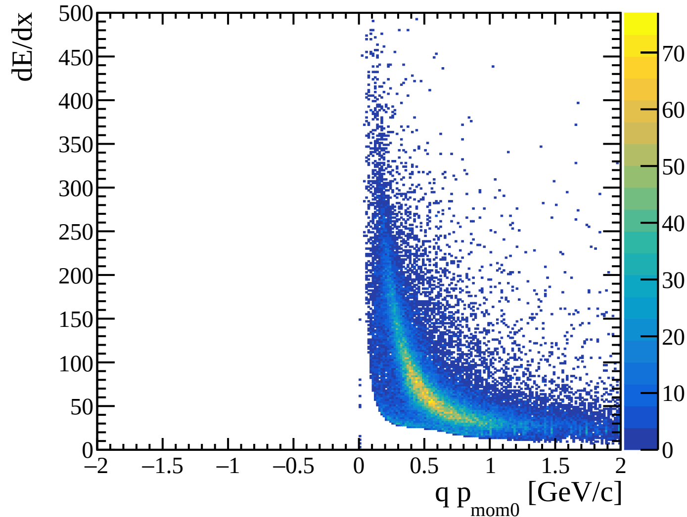
proton dE/dx vs signed momentum, tight cut
