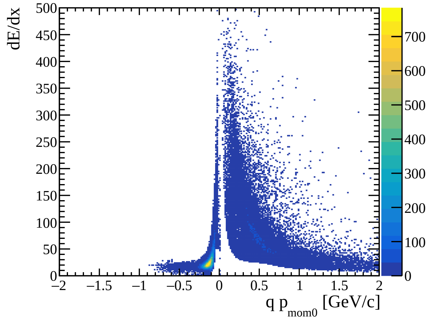
dE/dx vs signed momentum, Lambda peak
