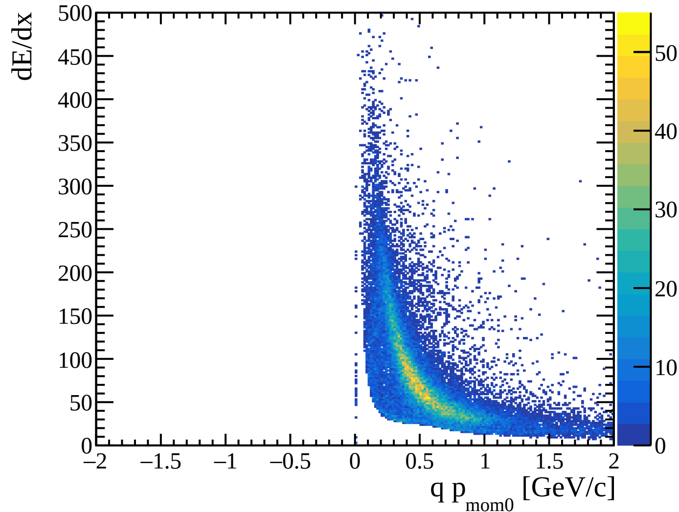
proton dE/dx vs signed momentum, Lambda peak
