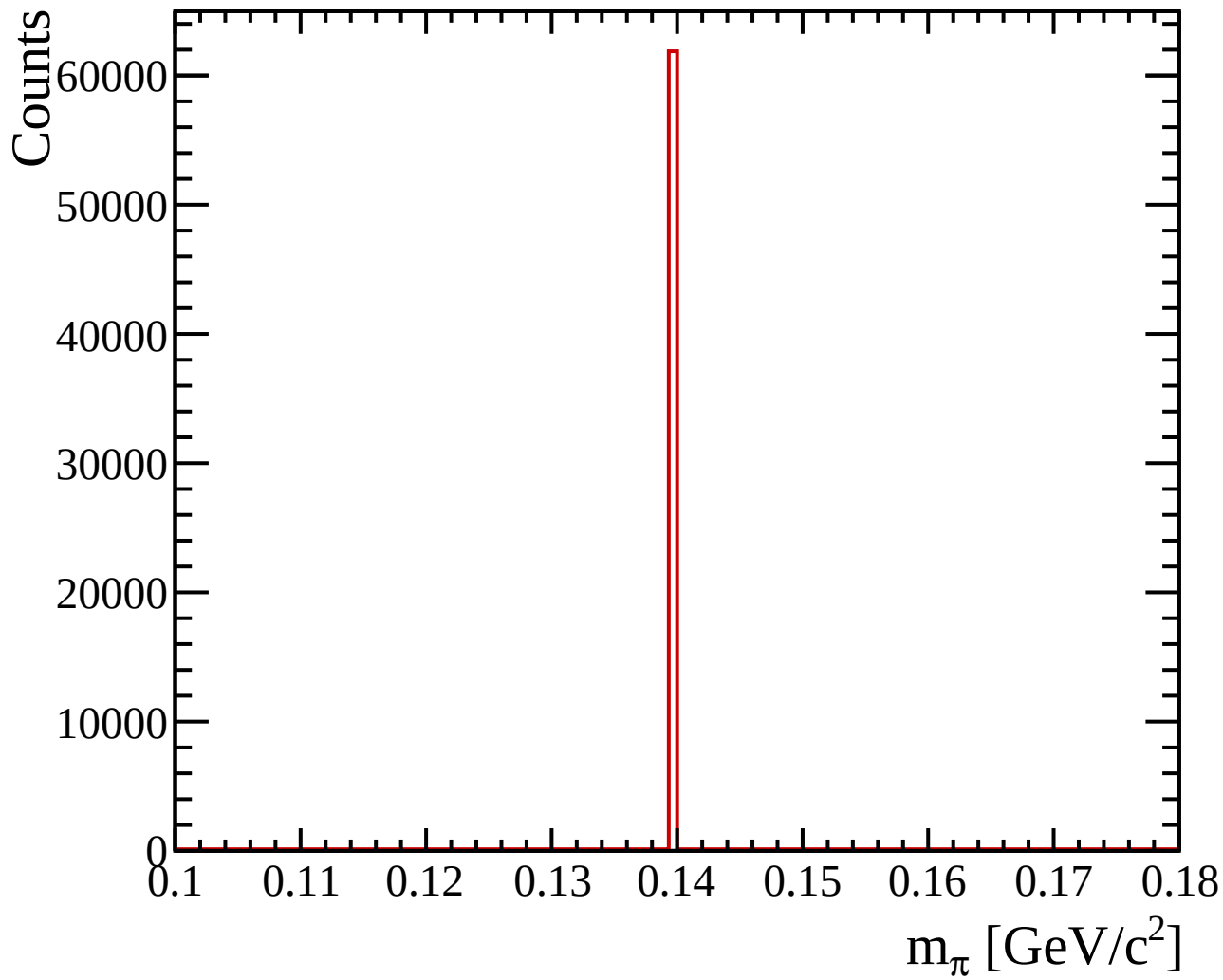
\pi^- candidate invariant mass, tight cut
