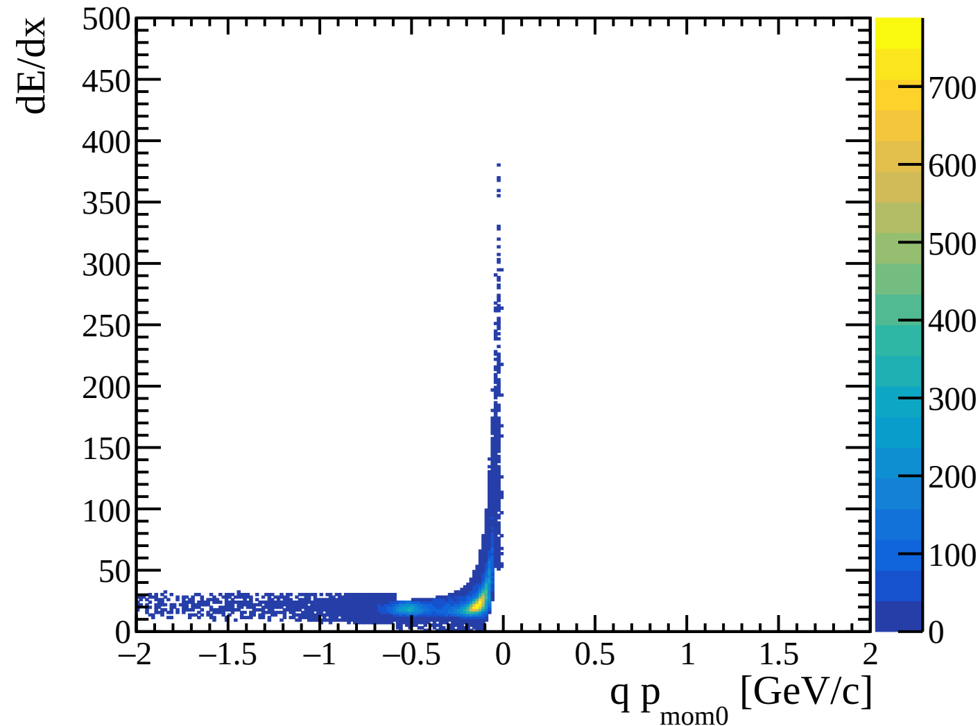
\pi^- dE/dx vs signed momentum, tight cut
