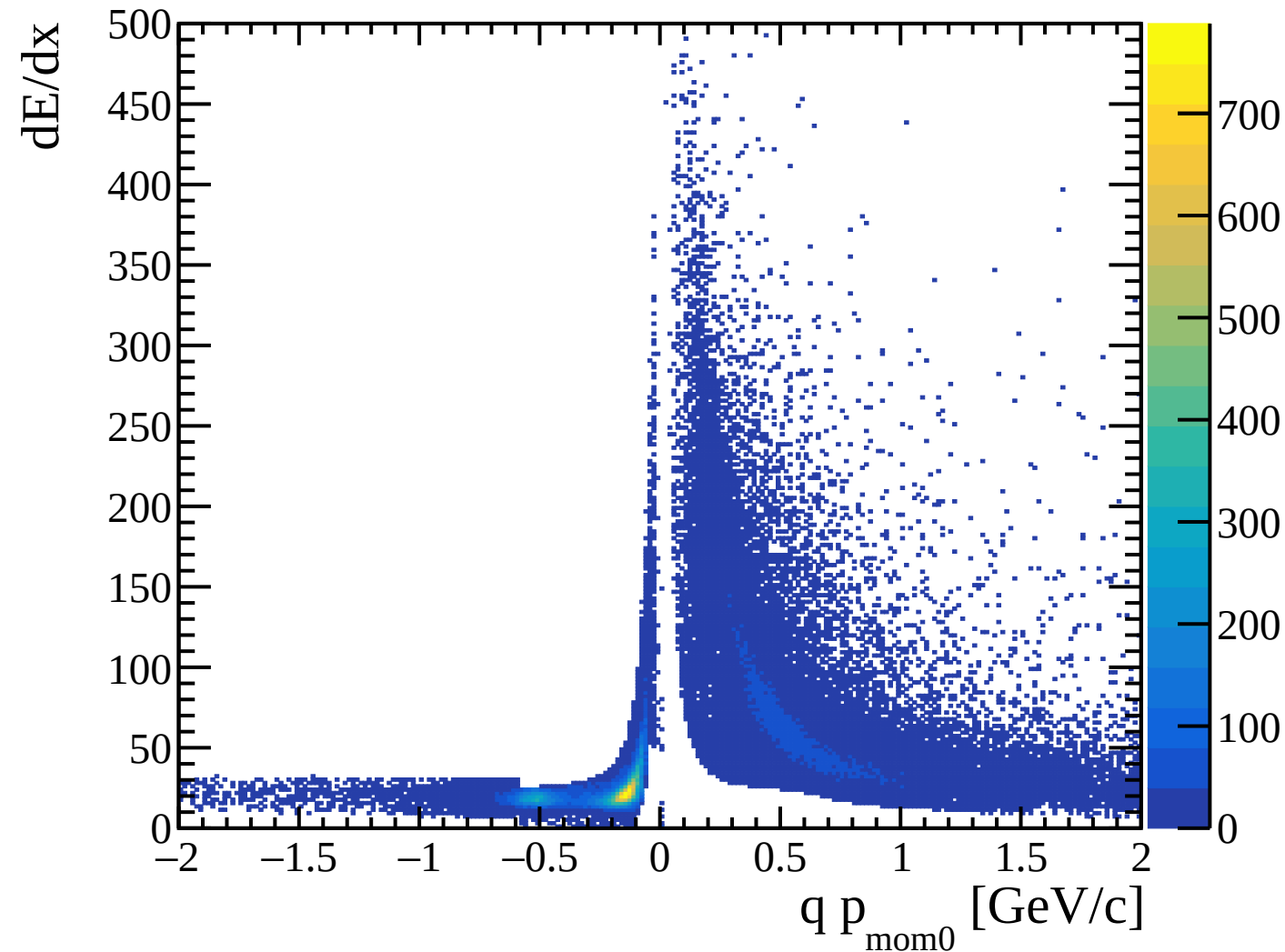
dE/dx vs signed momentum, tight cut
