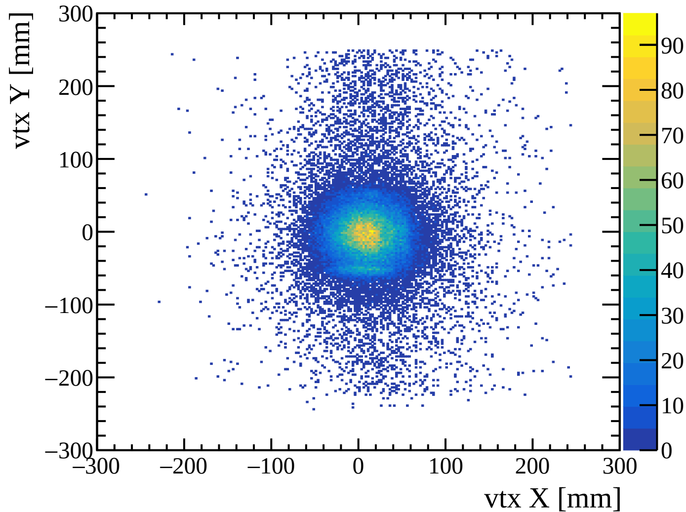
vertex, tight cut
