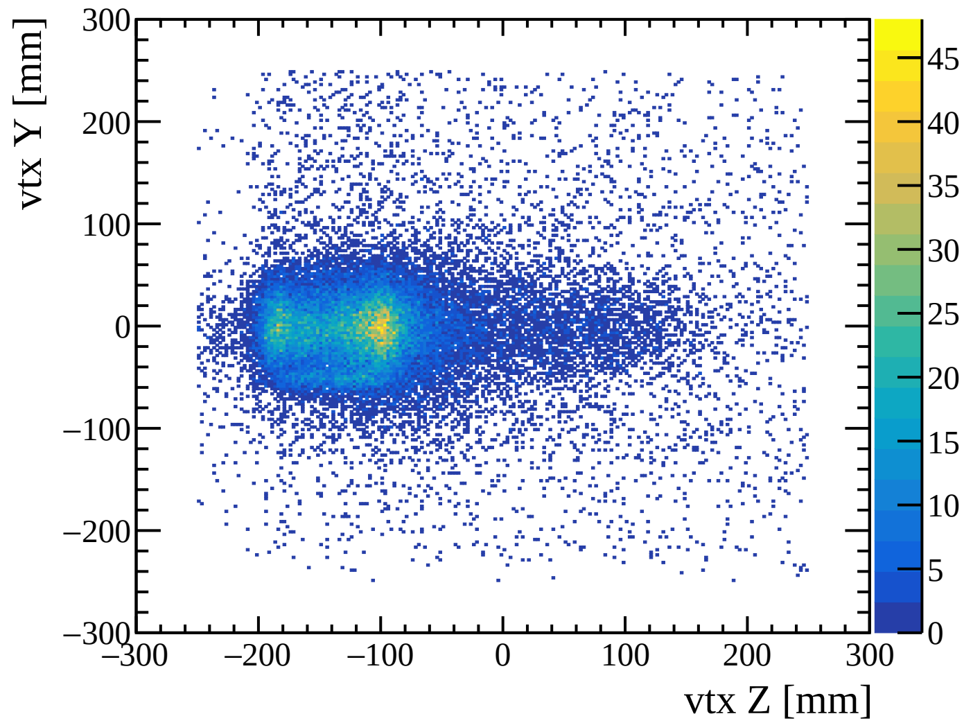
vertex, Lambda peak
