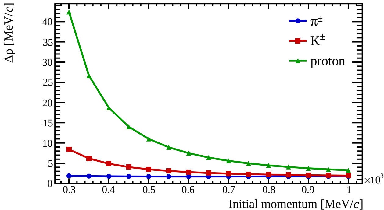
Momentum loss to the LH2 center
