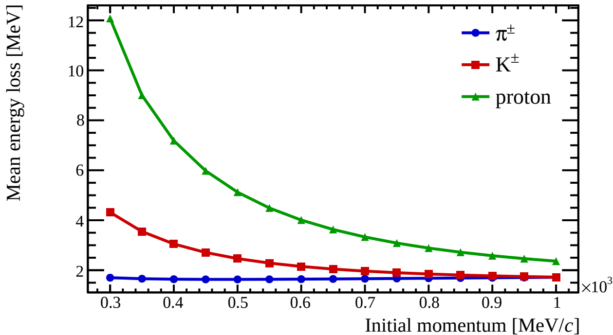
Energy loss to the LH2 center
