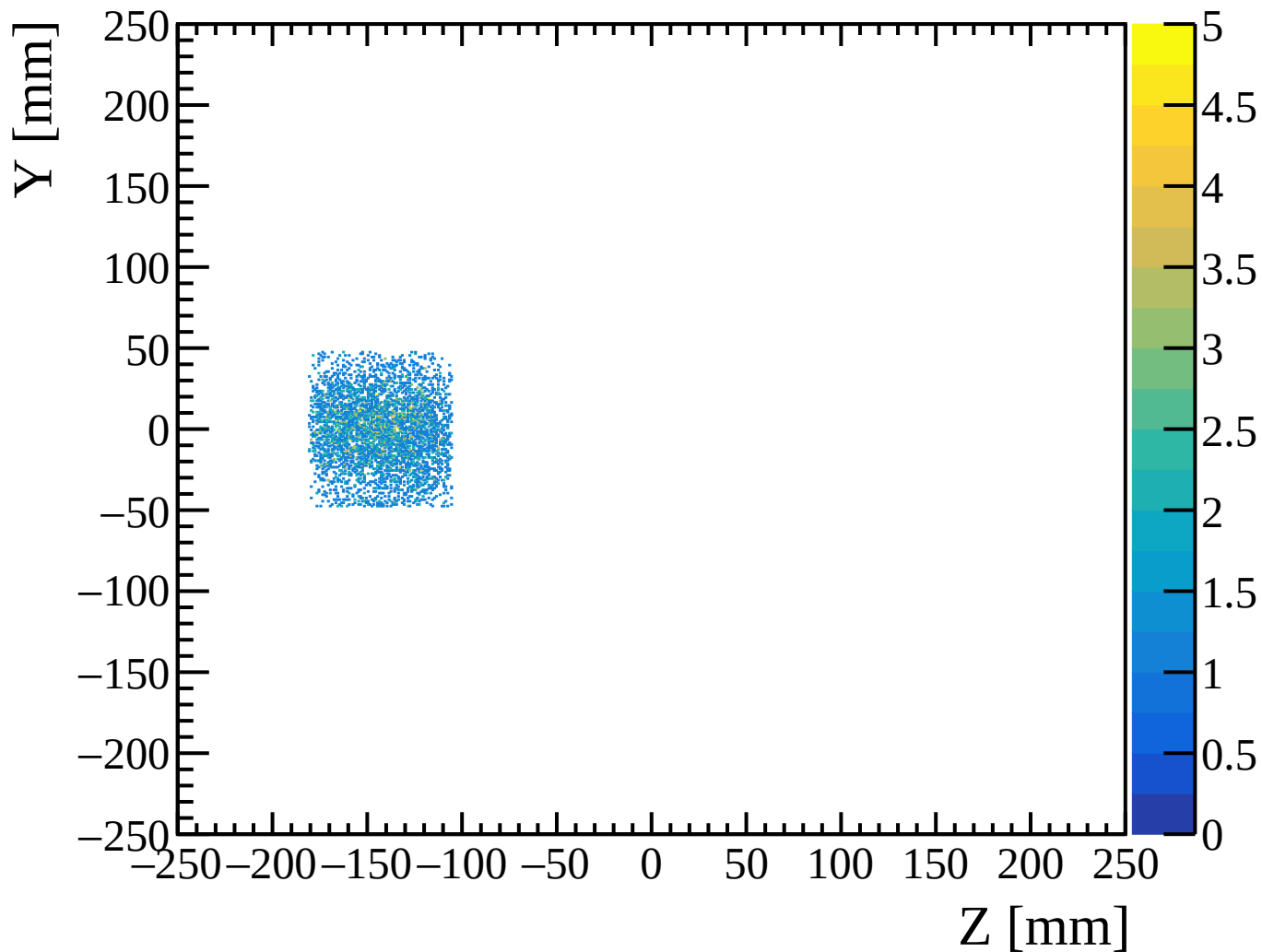
Reconstructed \Lambda production vertex (LH2 inside, M_X > 0.50 \text{ GeV}/c^2 )
