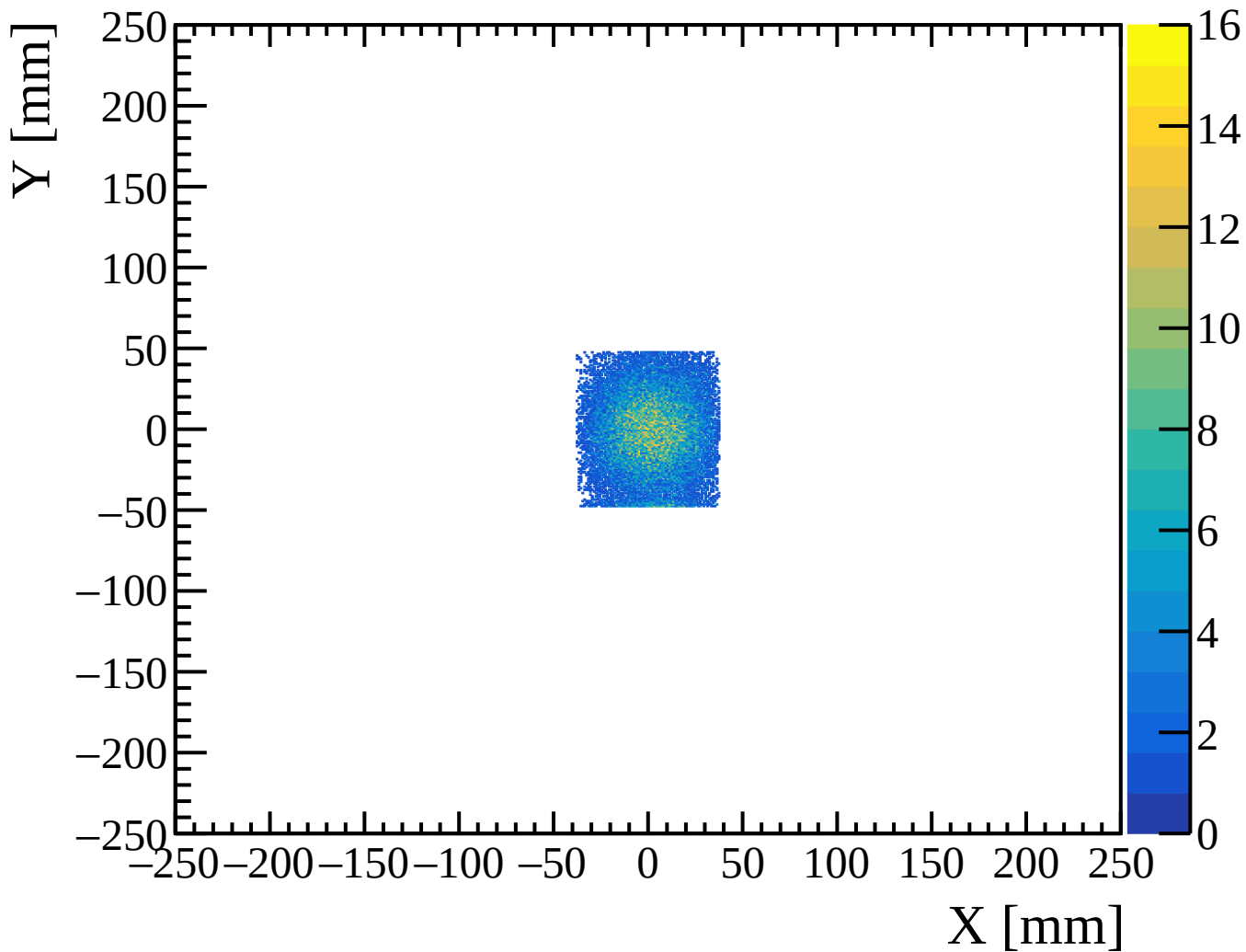
Reconstructed \Lambda production vertex (LH2 inside, no M_x cut)
