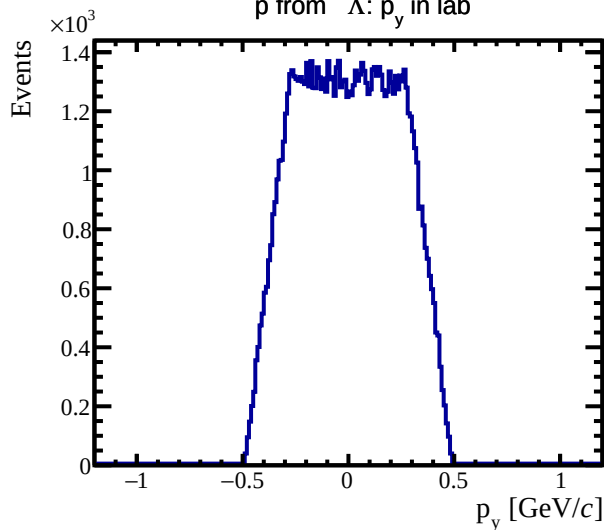
p from \Lambda : p_y in lab
