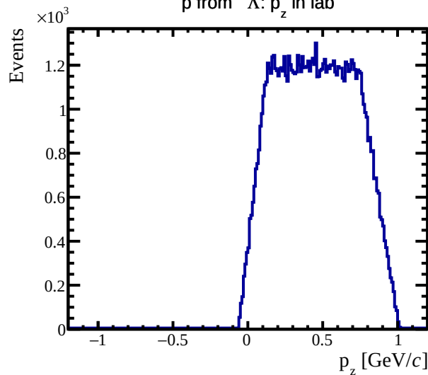
p from \Lambda : p_z in lab
