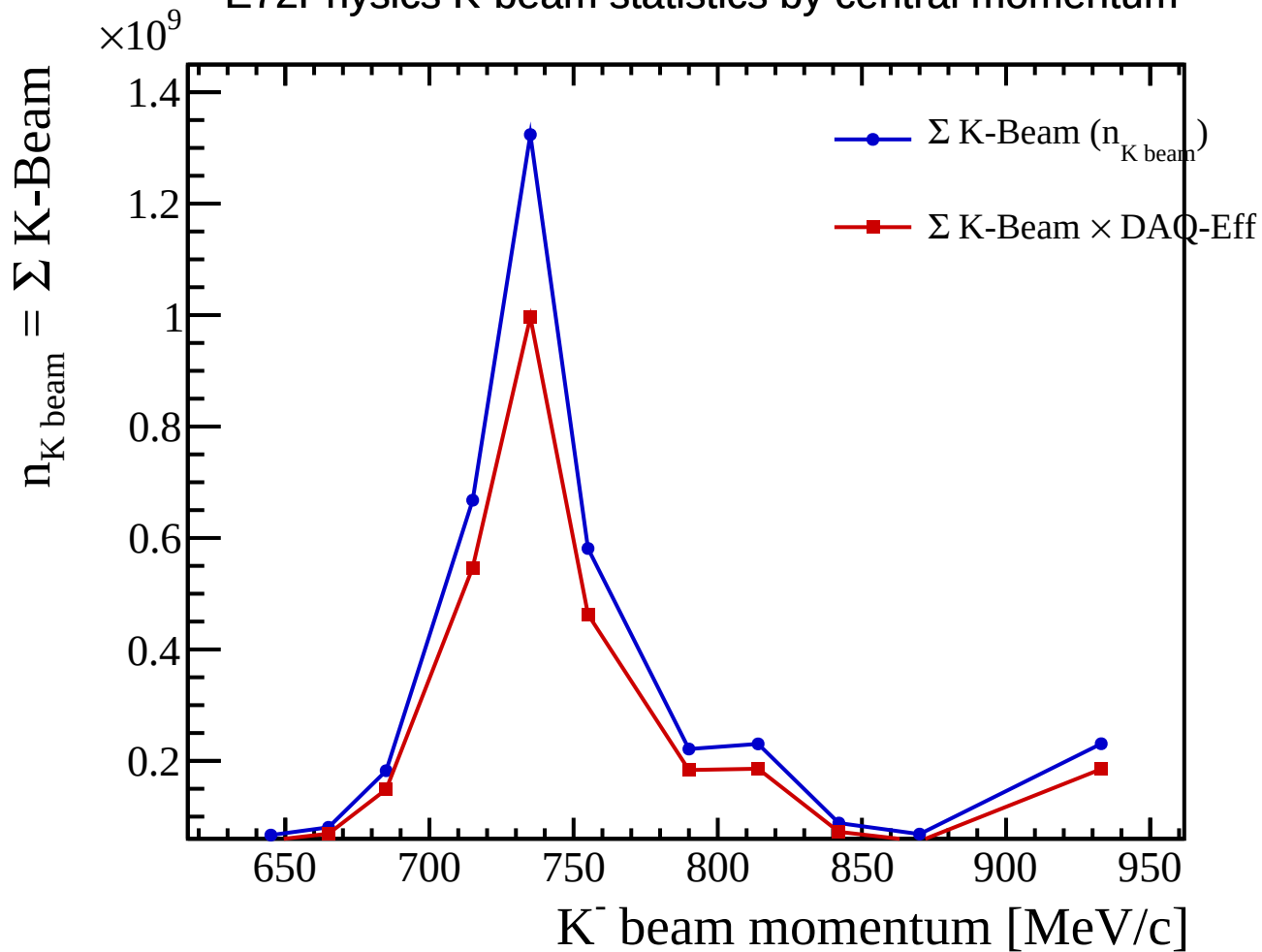
E72Physics K-beam statistics by central momentum
