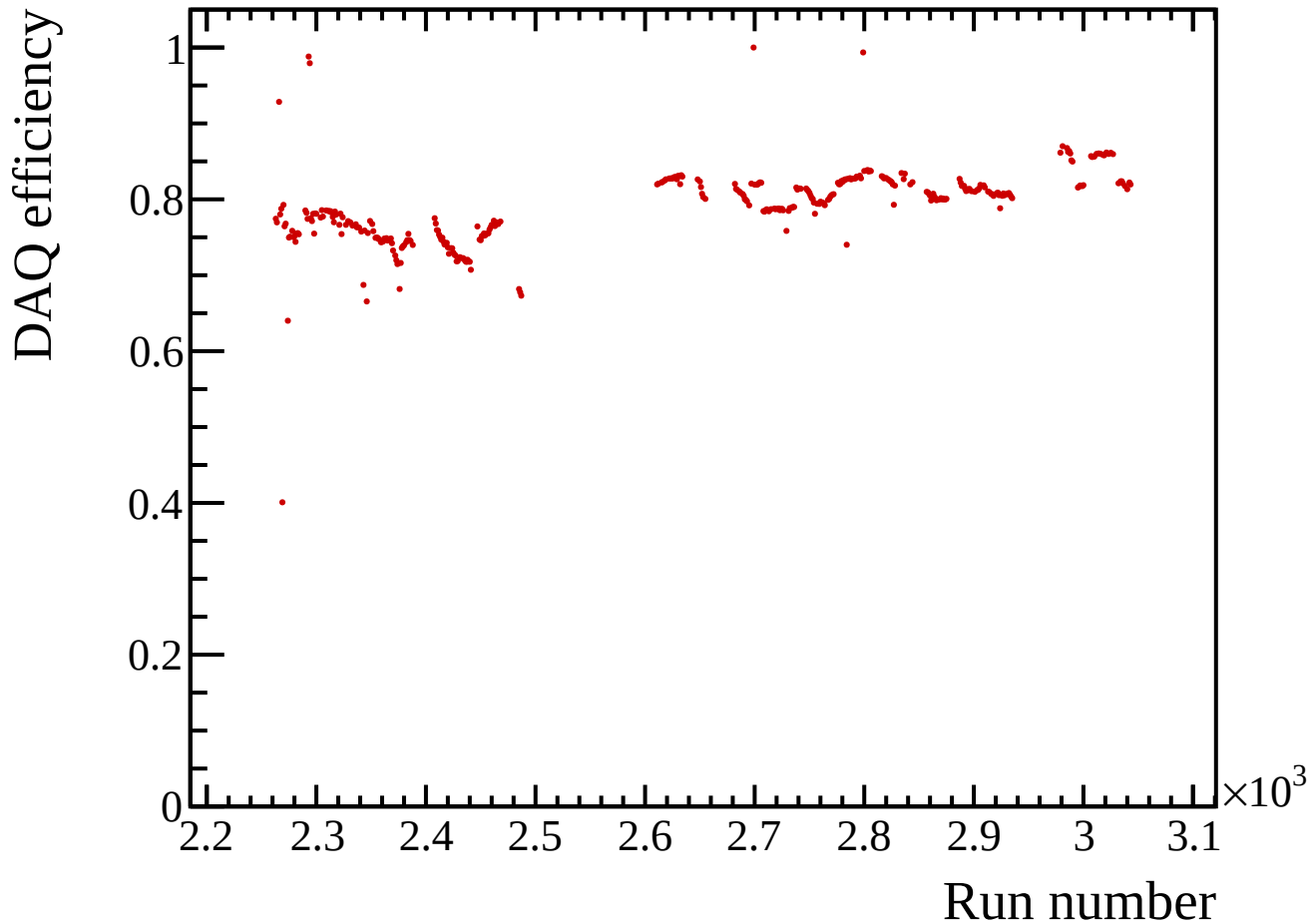
E72Physics run-by-run DAQ efficiency
