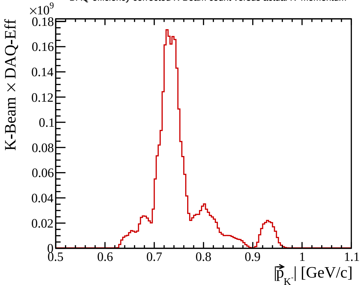
DAQ-efficiency corrected K-Beam count versus actual K^- momentum
