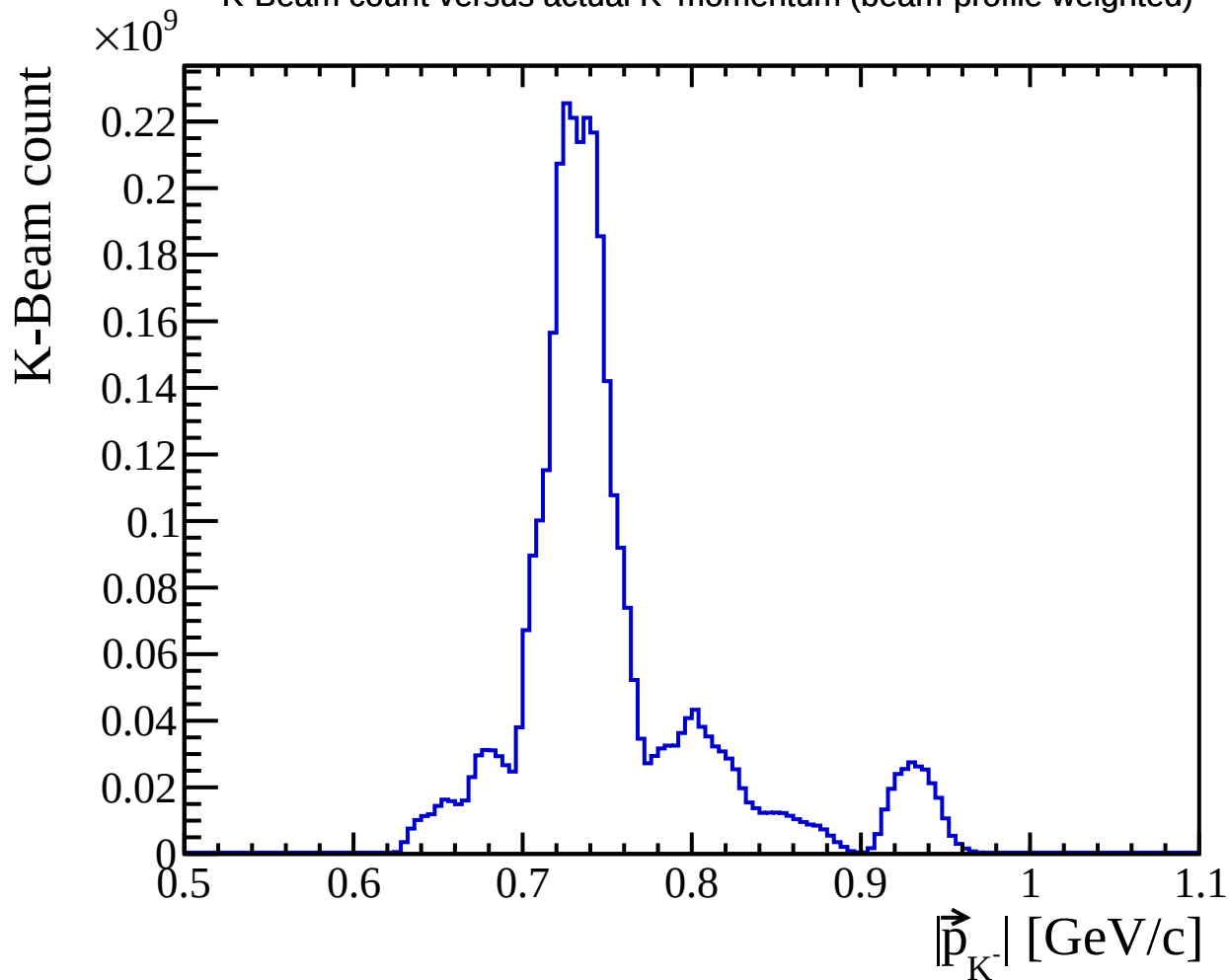
K-Beam count versus actual K^- momentum (beam-profile weighted)
