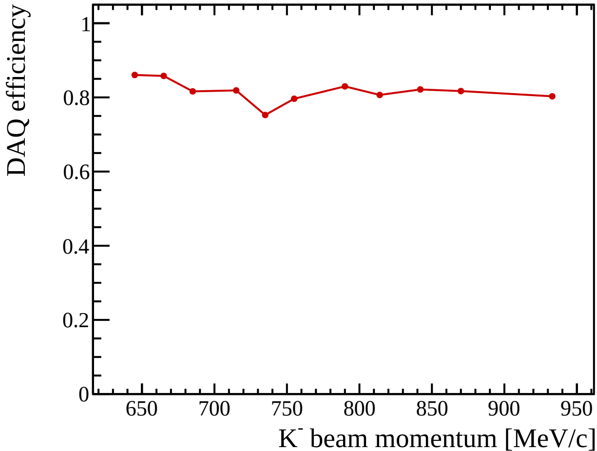
K-Beam-weighted DAQ efficiency by central momentum
